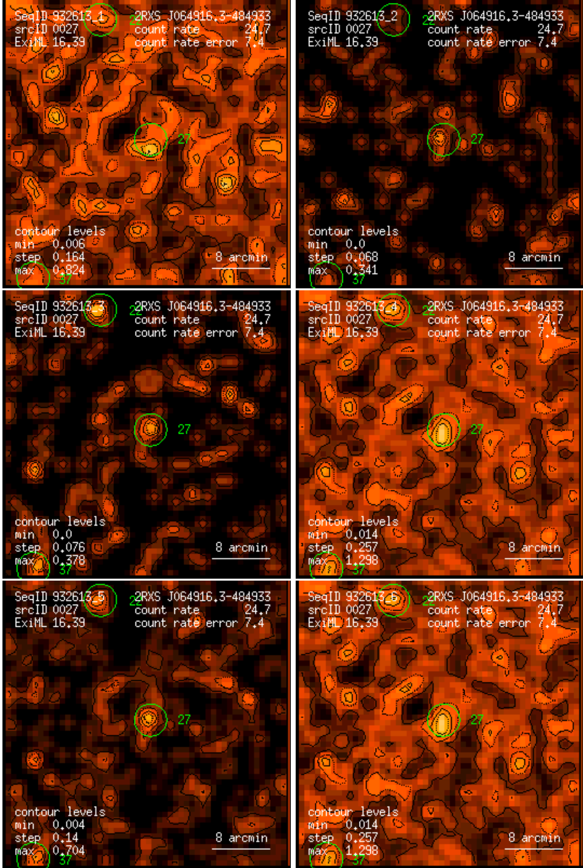
Figure 27: RASS 932613: detection 0027: band rate images, Gaussian filter: (1) PSPC channels 11 – 41, (2) 52 – 90, (3) 91 – 201, (4) 11 – 235, (5) 52 – 201, (6) 11 – 201. Broad band rates in counts/ks. Band rate contour levels in counts/ks/arcmin 2 .
