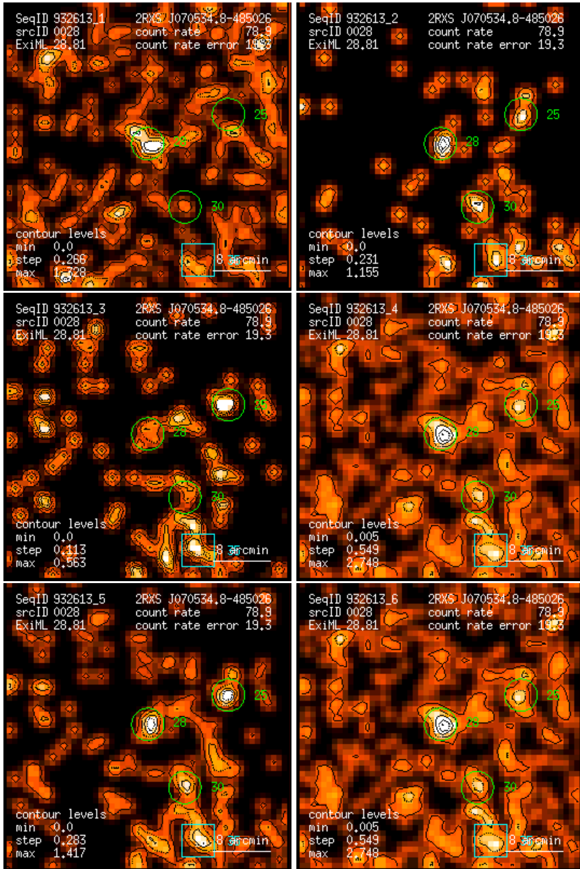
Figure 28: RASS 932613: detection 0028: band rate images, Gaussian filter: (1) PSPC channels 11 – 41, (2) 52 – 90, (3) 91 – 201, (4) 11 – 235, (5) 52 – 201, (6) 11 – 201. Broad band rates in counts/ks. Band rate contour levels in counts/ks/arcmin 2 .
