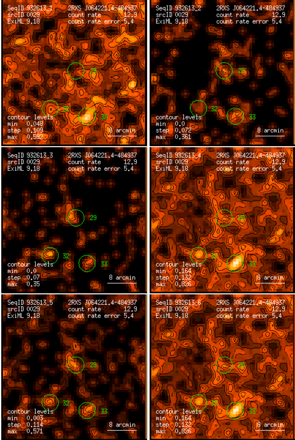
Figure 29: RASS 932613: detection 0029: band rate images, Gaussian filter: (1) PSPC channels 11 – 41, (2) 52 – 90, (3) 91 – 201, (4) 11 – 235, (5) 52 – 201, (6) 11 – 201. Broad band rates in counts/ks. Band rate contour levels in counts/ks/arcmin 2 .
