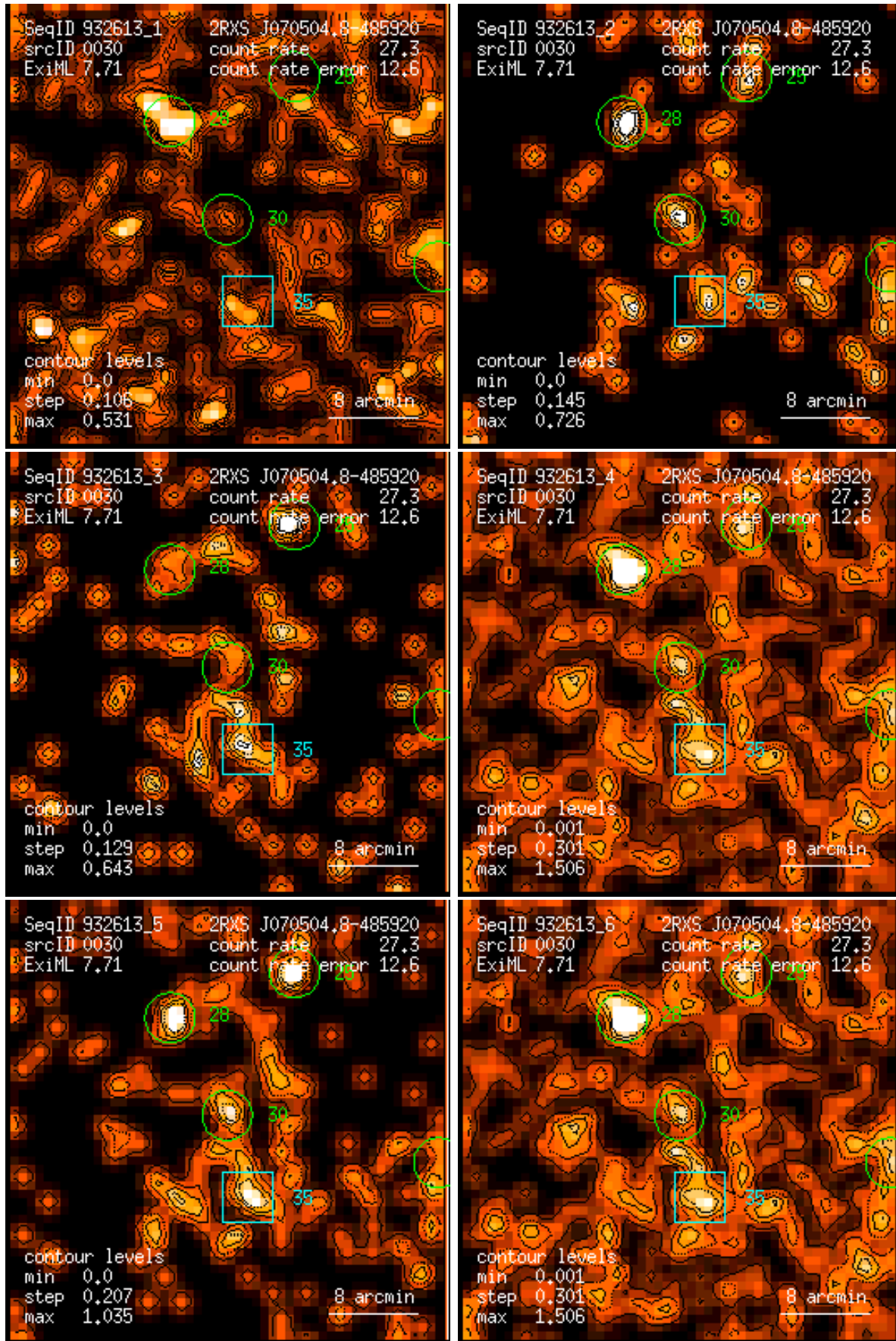
Figure 30: RASS 932613: detection 0030: band rate images, Gaussian filter: (1) PSPC channels 11 – 41, (2) 52 – 90, (3) 91 – 201, (4) 11 – 235, (5) 52 – 201, (6) 11 – 201. Broad band rates in counts/ks. Band rate contour levels in counts/ks/arcmin 2 .
