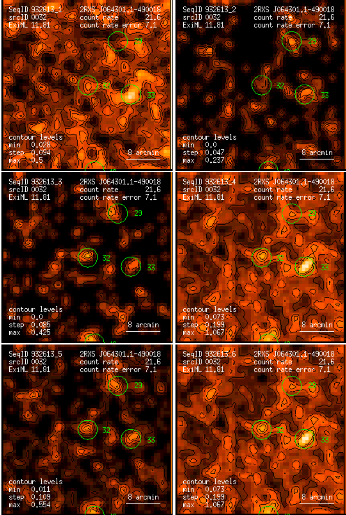
Figure 32: RASS 932613: detection 0032: band rate images, Gaussian filter: (1) PSPC channels 11 – 41, (2) 52 – 90, (3) 91 – 201, (4) 11 – 235, (5) 52 – 201, (6) 11 – 201. Broad band rates in counts/ks. Band rate contour levels in counts/ks/arcmin 2 .
