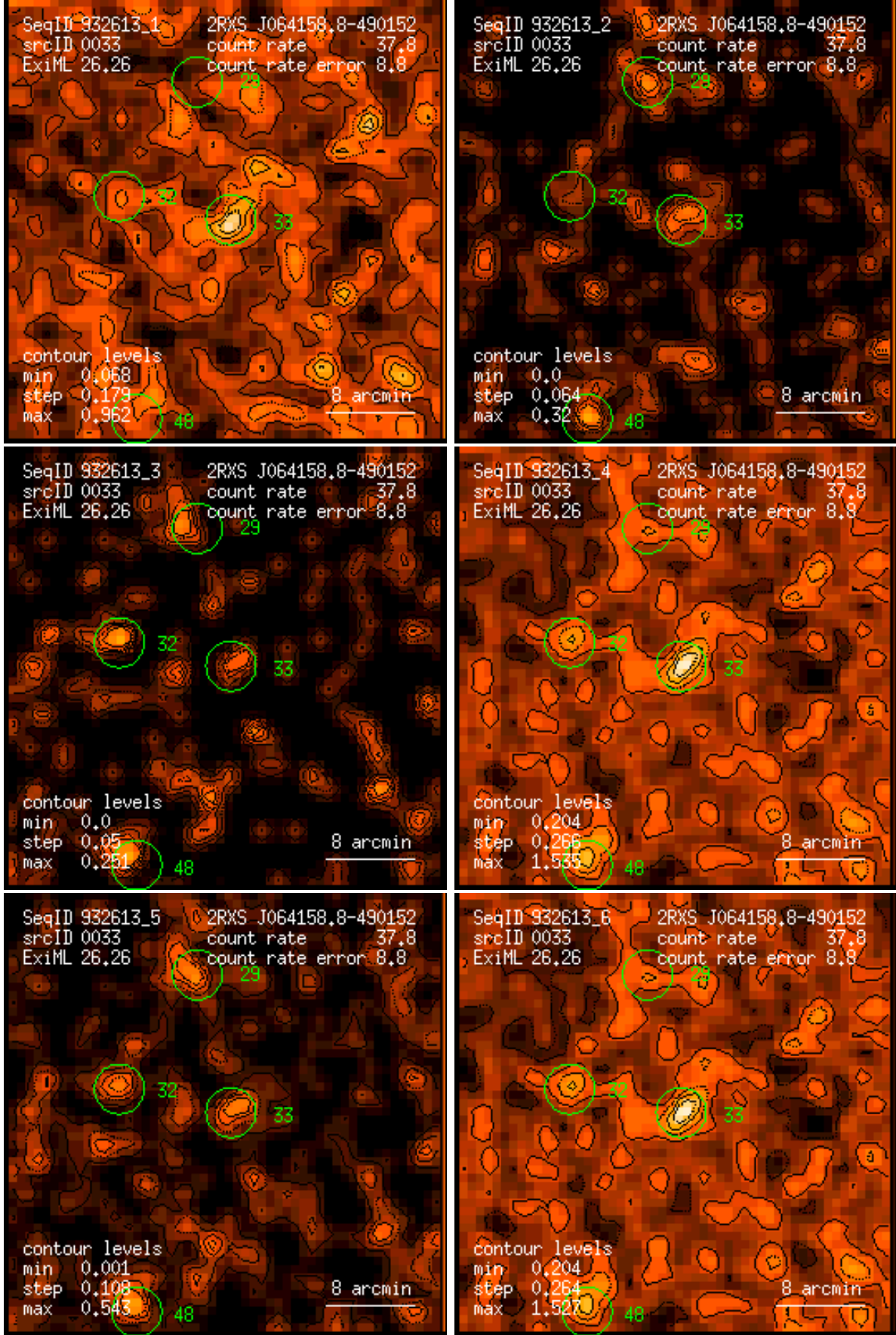
Figure 33: RASS 932613: detection 0033: band rate images, Gaussian filter: (1) PSPC channels 11 – 41, (2) 52 – 90, (3) 91 – 201, (4) 11 – 235, (5) 52 – 201, (6) 11 – 201. Broad band rates in counts/ks. Band rate contour levels in counts/ks/arcmin 2 .
