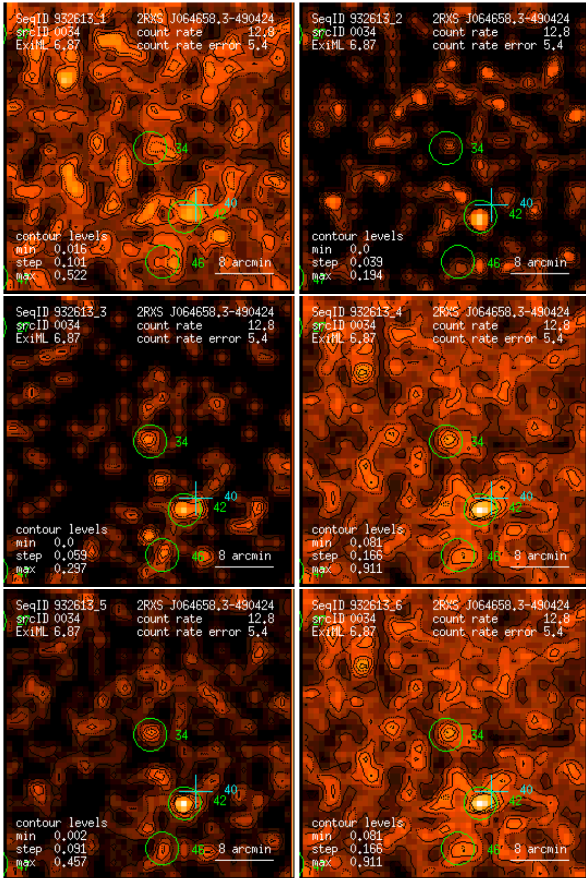
Figure 34: RASS 932613: detection 0034: band rate images, Gaussian filter: (1) PSPC channels 11 – 41, (2) 52 – 90, (3) 91 – 201, (4) 11 – 235, (5) 52 – 201, (6) 11 – 201. Broad band rates in counts/ks. Band rate contour levels in counts/ks/arcmin 2 .
