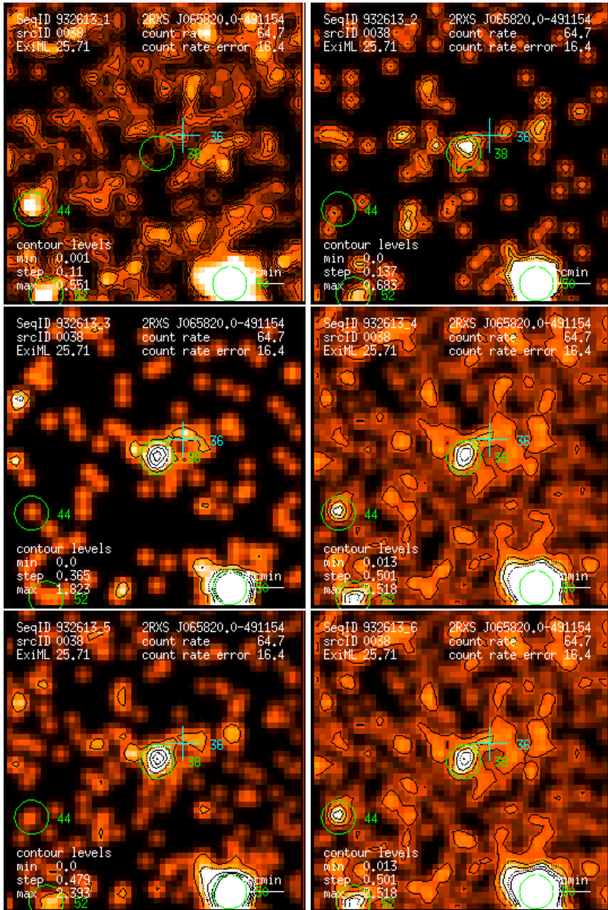
Figure 38: RASS 932613: detection 0038: band rate images, Gaussian filter: (1) PSPC channels 11 – 41, (2) 52 – 90, (3) 91 – 201, (4) 11 – 235, (5) 52 – 201, (6) 11 – 201. Broad band rates in counts/ks. Band rate contour levels in counts/ks/arcmin 2 .
