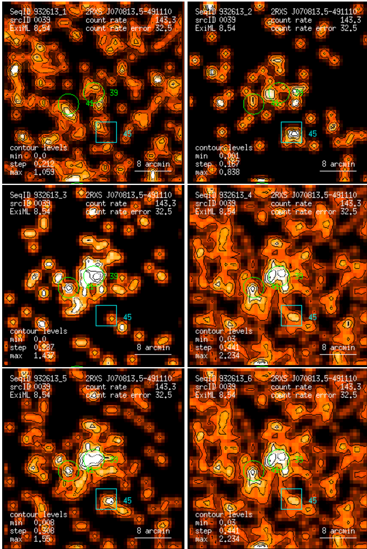
Figure 39: RASS 932613: detection 0039: band rate images, Gaussian filter: (1) PSPC channels 11 – 41, (2) 52 – 90, (3) 91 – 201, (4) 11 – 235, (5) 52 – 201, (6) 11 – 201. Broad band rates in counts/ks. Band rate contour levels in counts/ks/arcmin 2 .
