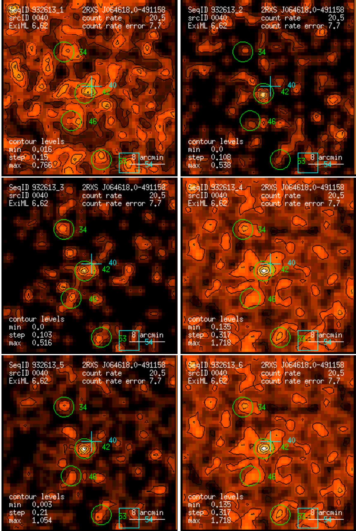
Figure 40: RASS 932613: detection 0040: band rate images, Gaussian filter: (1) PSPC channels 11 – 41, (2) 52 – 90, (3) 91 – 201, (4) 11 – 235, (5) 52 – 201, (6) 11 – 201. Broad band rates in counts/ks. Band rate contour levels in counts/ks/arcmin 2 .
