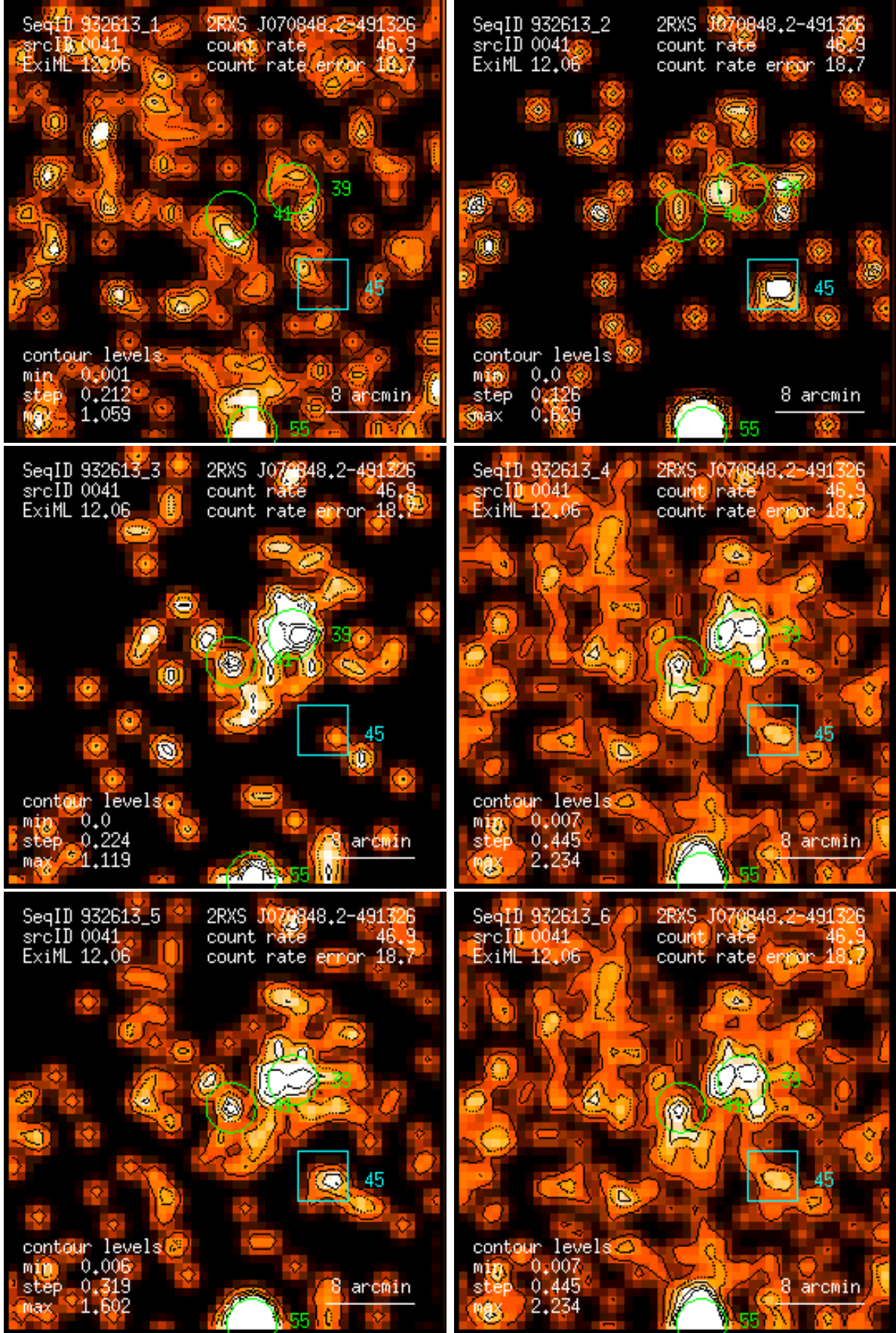
Figure 41: RASS 932613: detection 0041: band rate images, Gaussian filter: (1) PSPC channels 11 – 41, (2) 52 – 90, (3) 91 – 201, (4) 11 – 235, (5) 52 – 201, (6) 11 – 201. Broad band rates in counts/ks. Band rate contour levels in counts/ks/arcmin 2 .
