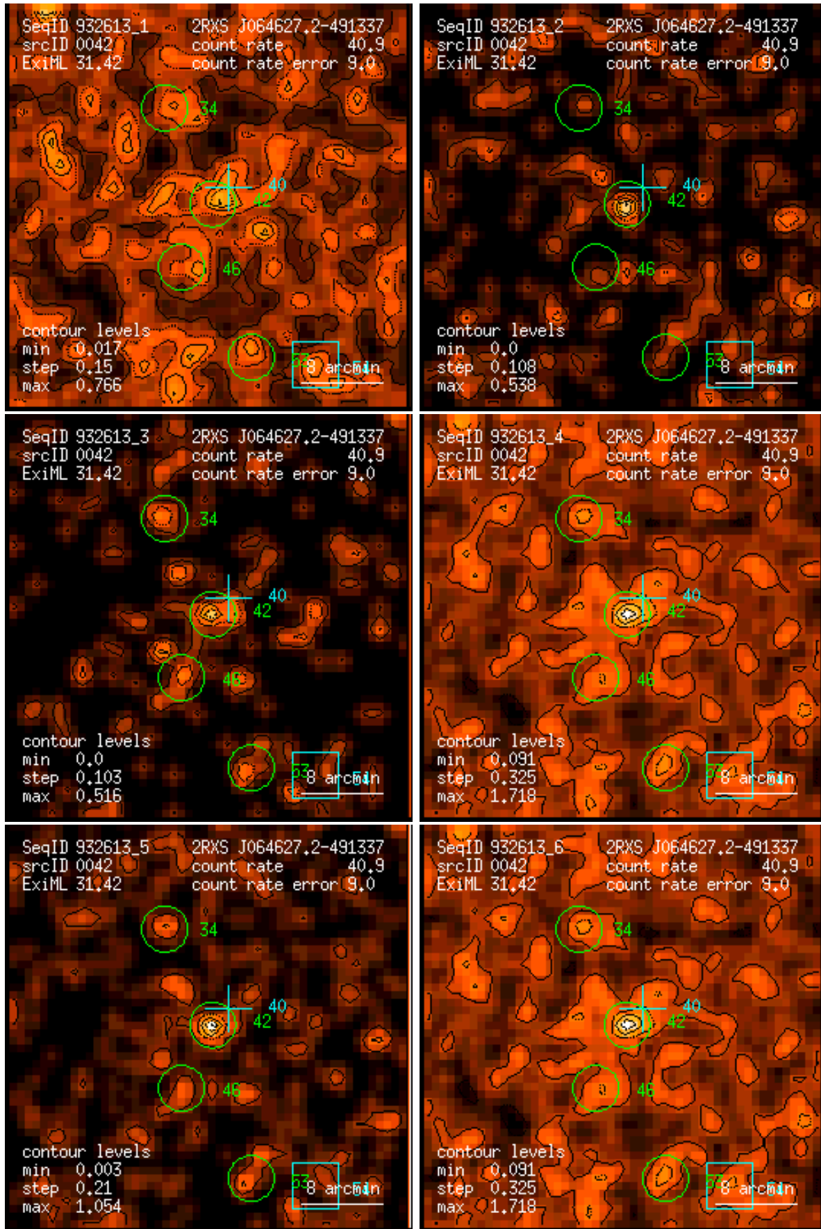
Figure 42: RASS 932613: detection 0042: band rate images, Gaussian filter: (1) PSPC channels 11 – 41, (2) 52 – 90, (3) 91 – 201, (4) 11 – 235, (5) 52 – 201, (6) 11 – 201. Broad band rates in counts/ks. Band rate contour levels in counts/ks/arcmin 2 .
