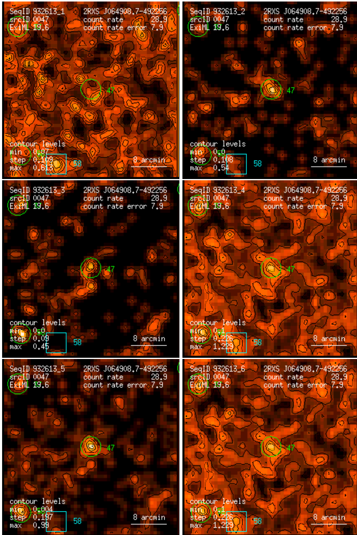
Figure 47: RASS 932613: detection 0047: band rate images, Gaussian filter: (1) PSPC channels 11 – 41, (2) 52 – 90, (3) 91 – 201, (4) 11 – 235, (5) 52 – 201, (6) 11 – 201. Broad band rates in counts/ks. Band rate contour levels in counts/ks/arcmin 2 .
