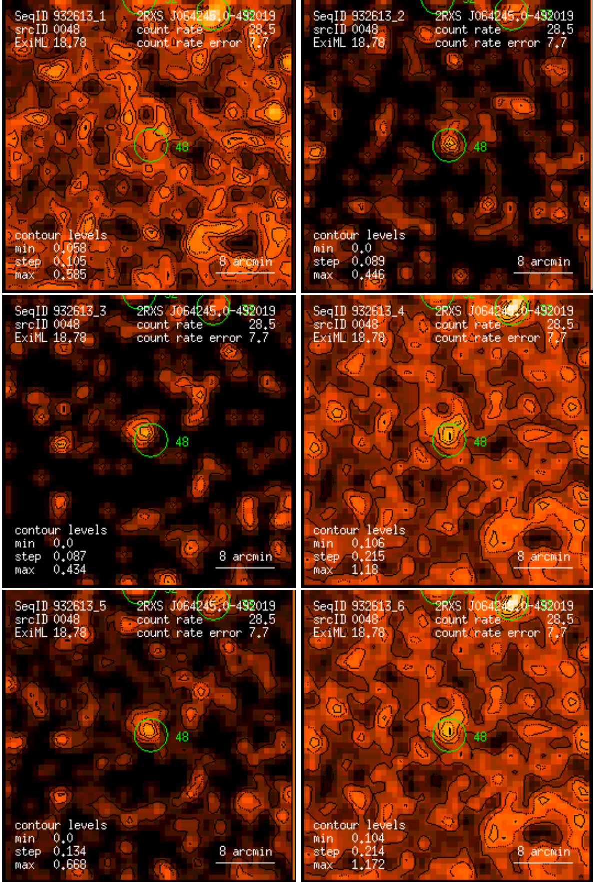
Figure 48: RASS 932613: detection 0048: band rate images, Gaussian filter: (1) PSPC channels 11 – 41, (2) 52 – 90, (3) 91 – 201, (4) 11 – 235, (5) 52 – 201, (6) 11 – 201. Broad band rates in counts/ks. Band rate contour levels in counts/ks/arcmin 2 .
