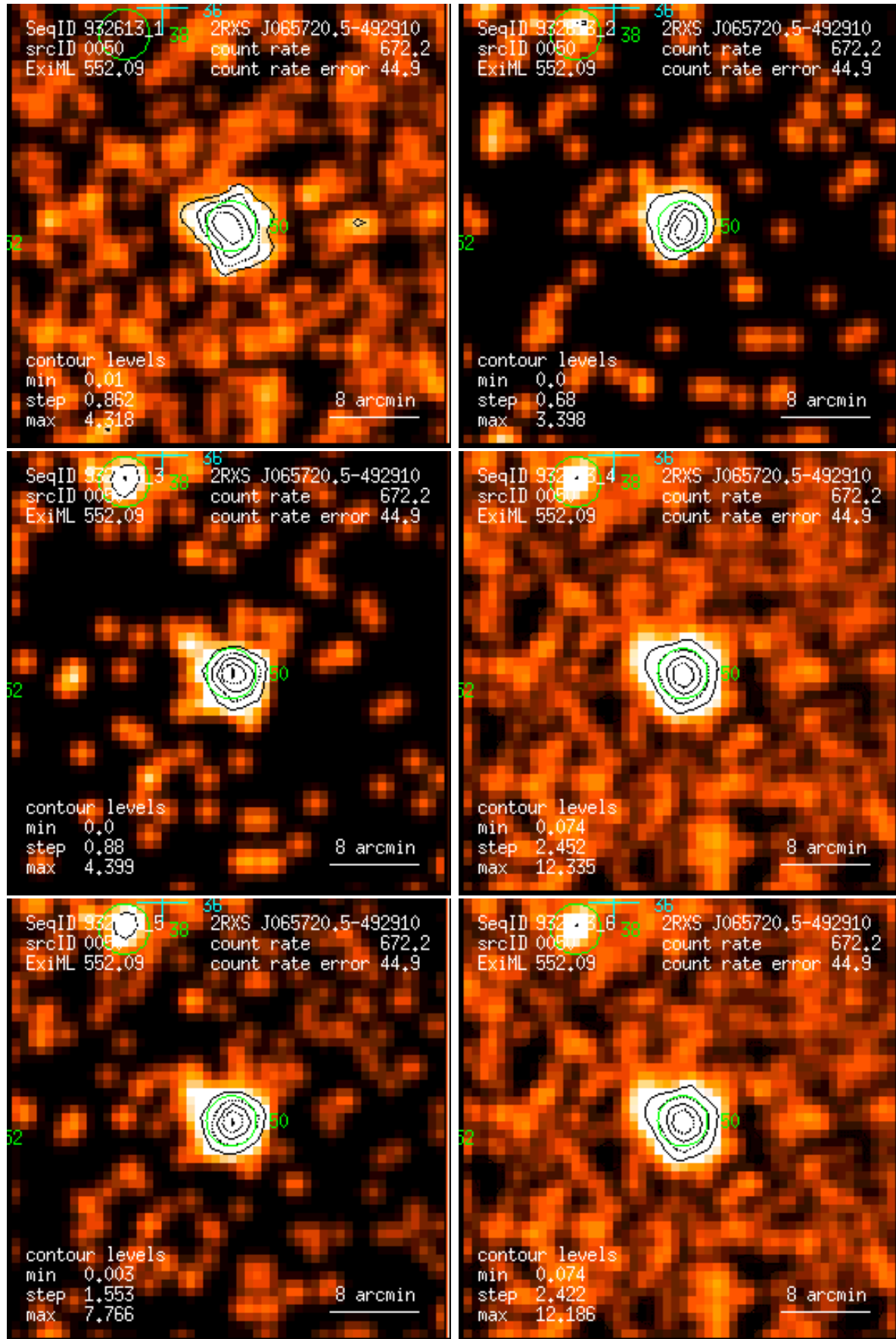
Figure 50: RASS 932613: detection 0050: band rate images, Gaussian filter: (1) PSPC channels 11 – 41, (2) 52 – 90, (3) 91 – 201, (4) 11 – 235, (5) 52 – 201, (6) 11 – 201. Broad band rates in counts/ks. Band rate contour levels in counts/ks/arcmin 2 .
