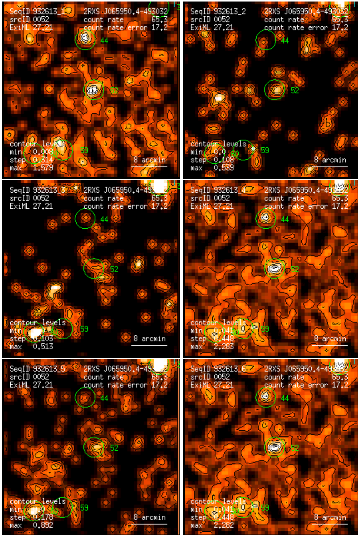
Figure 52: RASS 932613: detection 0052: band rate images, Gaussian filter: (1) PSPC channels 11 – 41, (2) 52 – 90, (3) 91 – 201, (4) 11 – 235, (5) 52 – 201, (6) 11 – 201. Broad band rates in counts/ks. Band rate contour levels in counts/ks/arcmin 2 .
