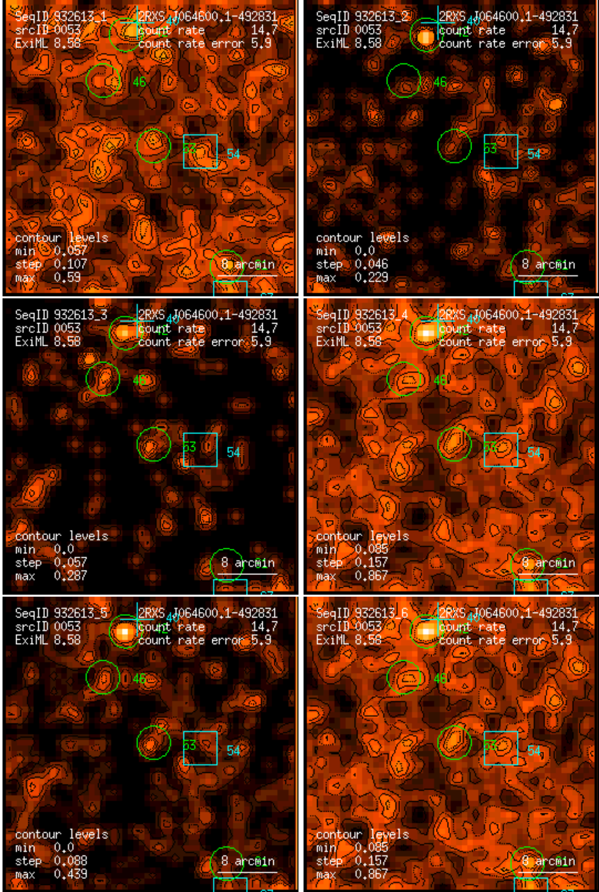
Figure 53: RASS 932613: detection 0053: band rate images, Gaussian filter: (1) PSPC channels 11 – 41, (2) 52 – 90, (3) 91 – 201, (4) 11 – 235, (5) 52 – 201, (6) 11 – 201. Broad band rates in counts/ks. Band rate contour levels in counts/ks/arcmin 2 .
