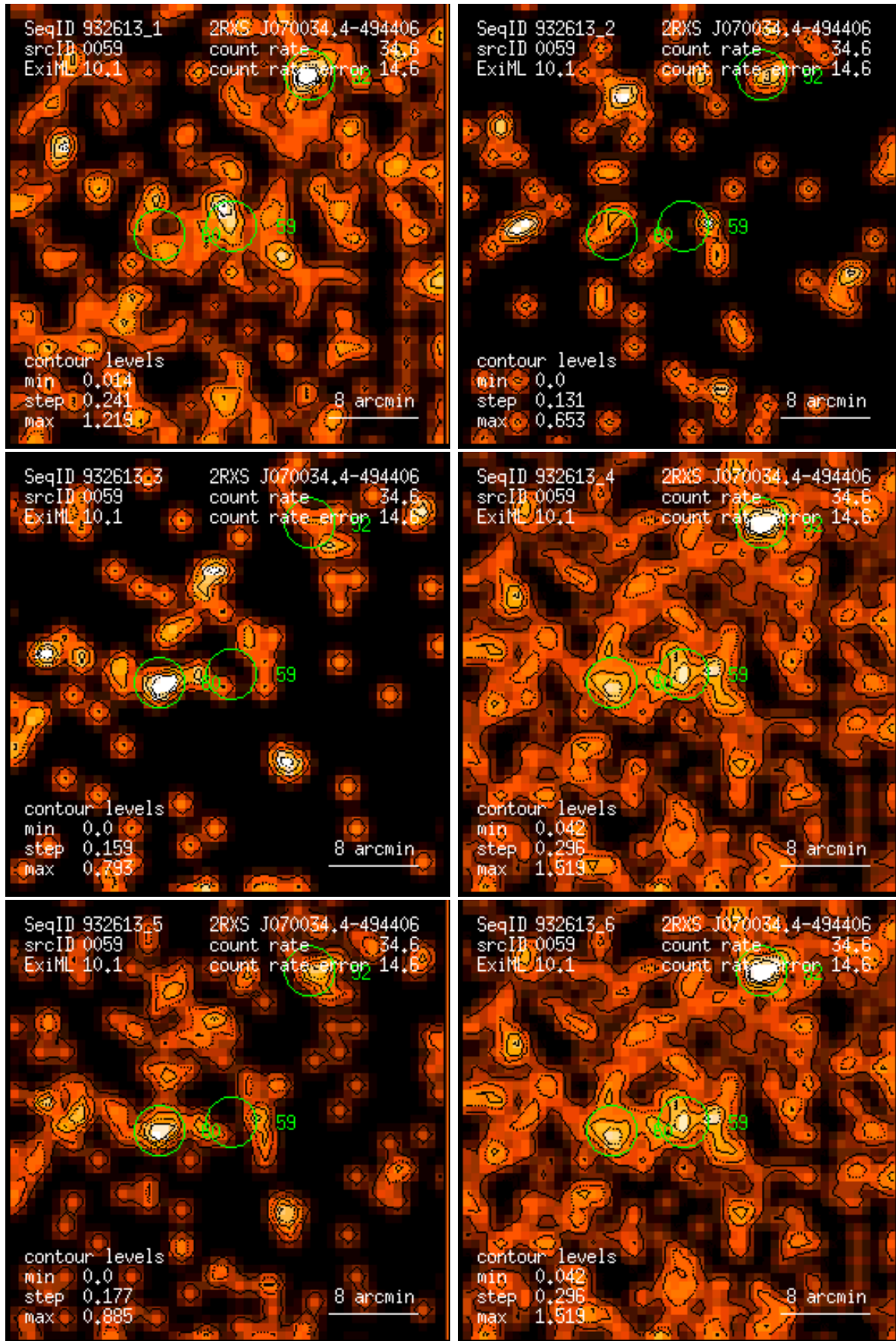
Figure 59: RASS 932613: detection 0059: band rate images, Gaussian filter: (1) PSPC channels 11 – 41, (2) 52 – 90, (3) 91 – 201, (4) 11 – 235, (5) 52 – 201, (6) 11 – 201. Broad band rates in counts/ks. Band rate contour levels in counts/ks/arcmin 2 .
