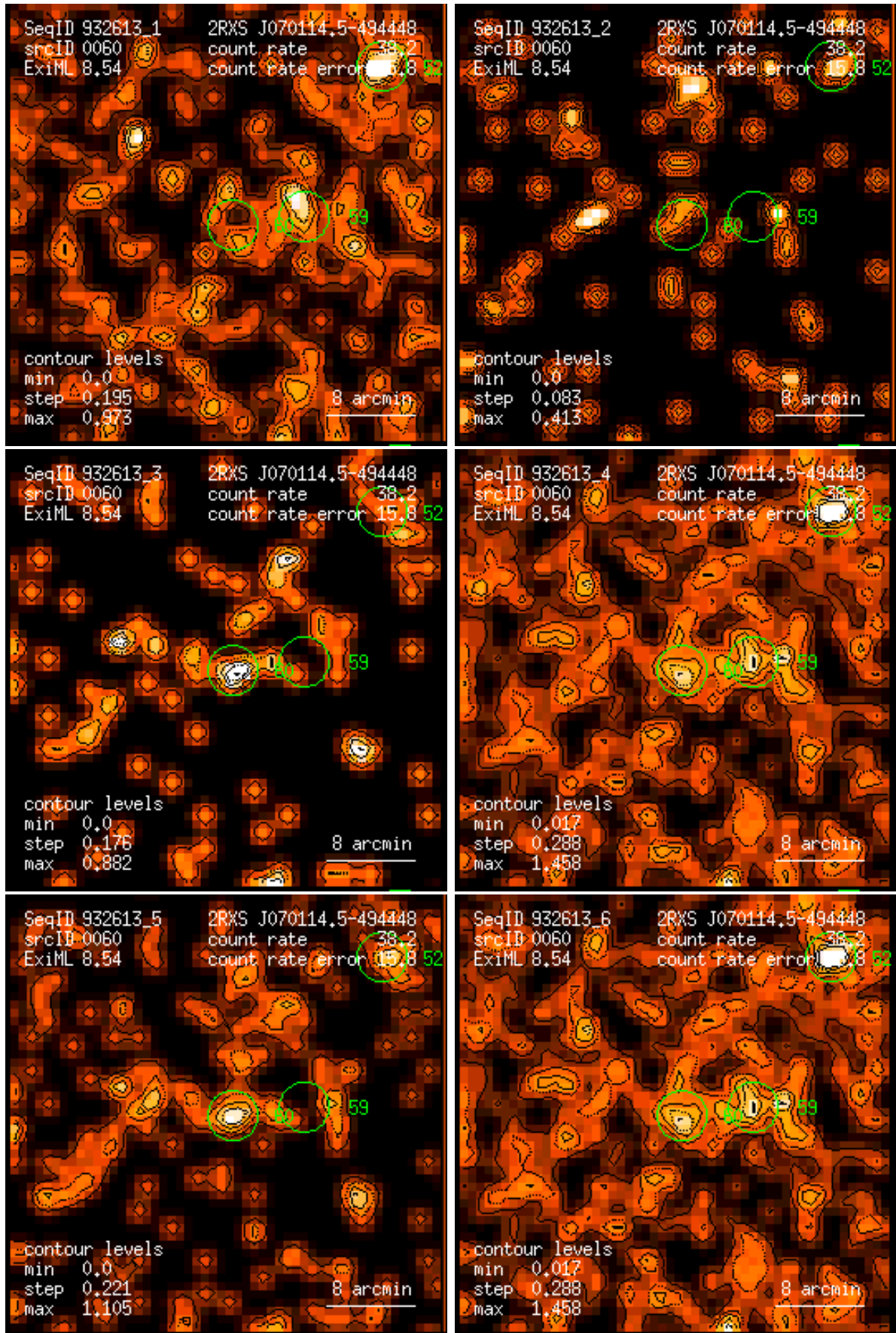
Figure 60: RASS 932613: detection 0060: band rate images, Gaussian filter: (1) PSPC channels 11 – 41, (2) 52 – 90, (3) 91 – 201, (4) 11 – 235, (5) 52 – 201, (6) 11 – 201. Broad band rates in counts/ks. Band rate contour levels in counts/ks/arcmin 2 .
