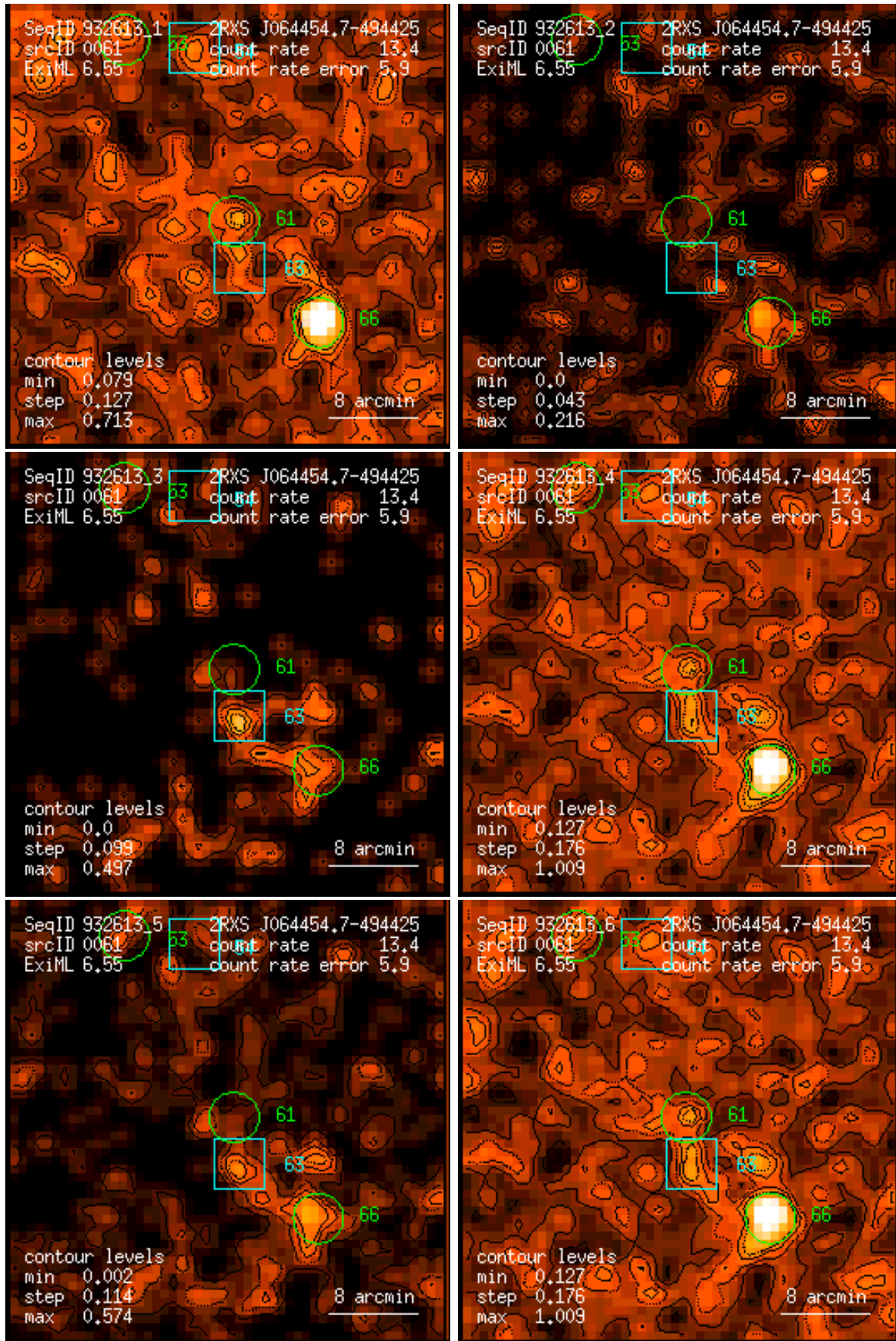
Figure 61: RASS 932613: detection 0061: band rate images, Gaussian filter: (1) PSPC channels 11 – 41, (2) 52 – 90, (3) 91 – 201, (4) 11 – 235, (5) 52 – 201, (6) 11 – 201. Broad band rates in counts/ks. Band rate contour levels in counts/ks/arcmin 2 .
