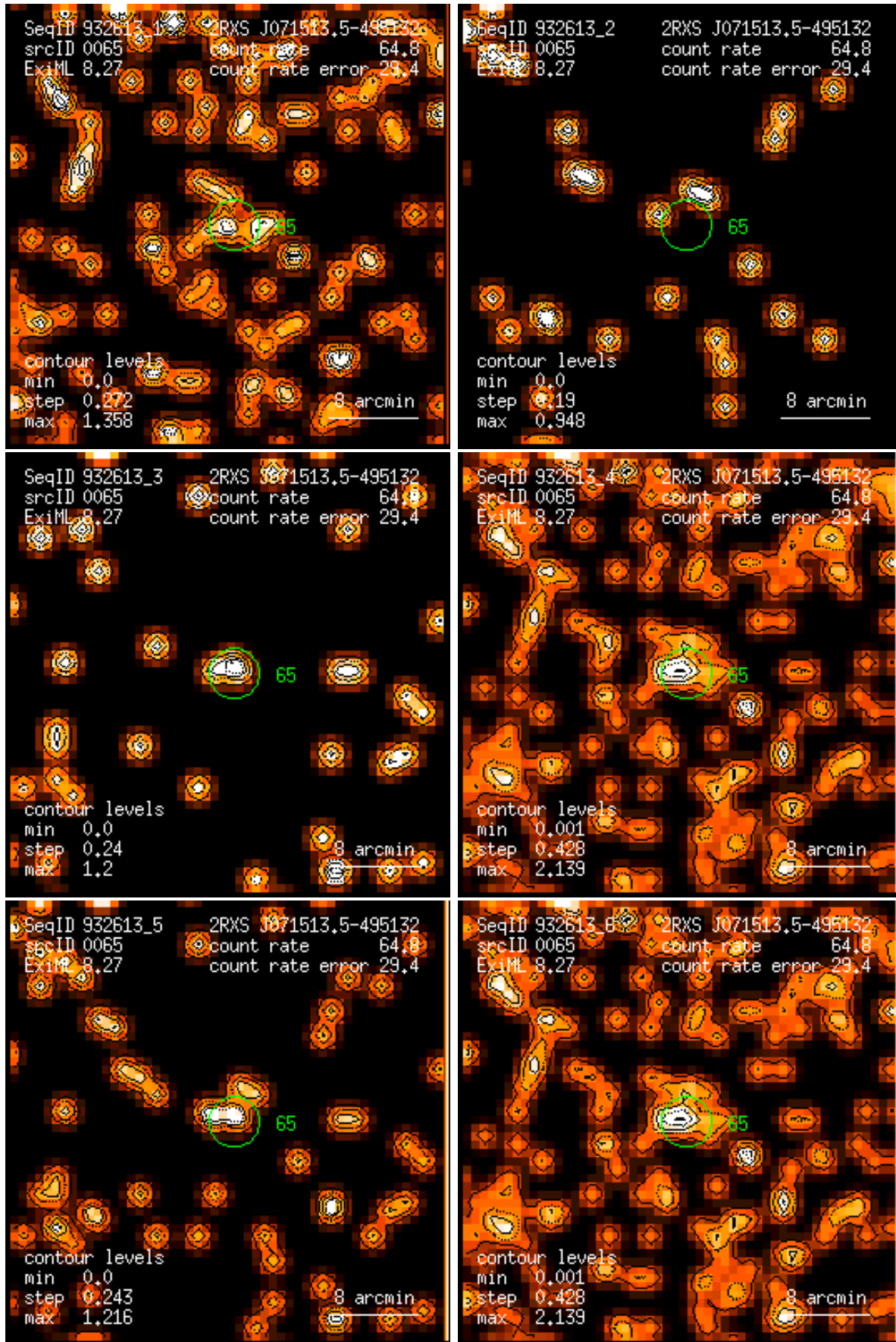
Figure 65: RASS 932613: detection 0065: band rate images, Gaussian filter: (1) PSPC channels 11 – 41, (2) 52 – 90, (3) 91 – 201, (4) 11 – 235, (5) 52 – 201, (6) 11 – 201. Broad band rates in counts/ks. Band rate contour levels in counts/ks/arcmin 2 .
