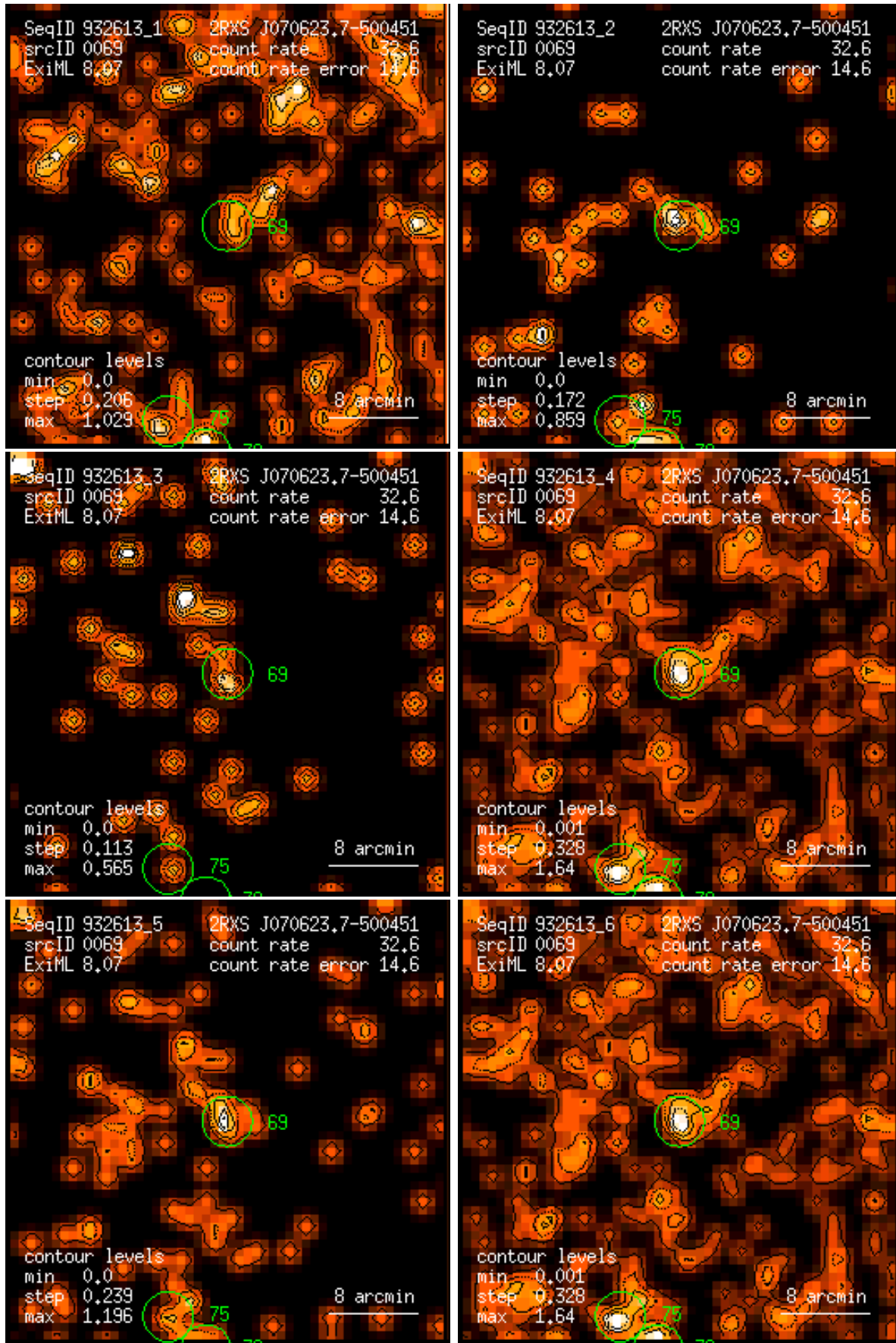
Figure 69: RASS 932613: detection 0069: band rate images, Gaussian filter: (1) PSPC channels 11 – 41, (2) 52 – 90, (3) 91 – 201, (4) 11 – 235, (5) 52 – 201, (6) 11 – 201. Broad band rates in counts/ks. Band rate contour levels in counts/ks/arcmin 2 .
