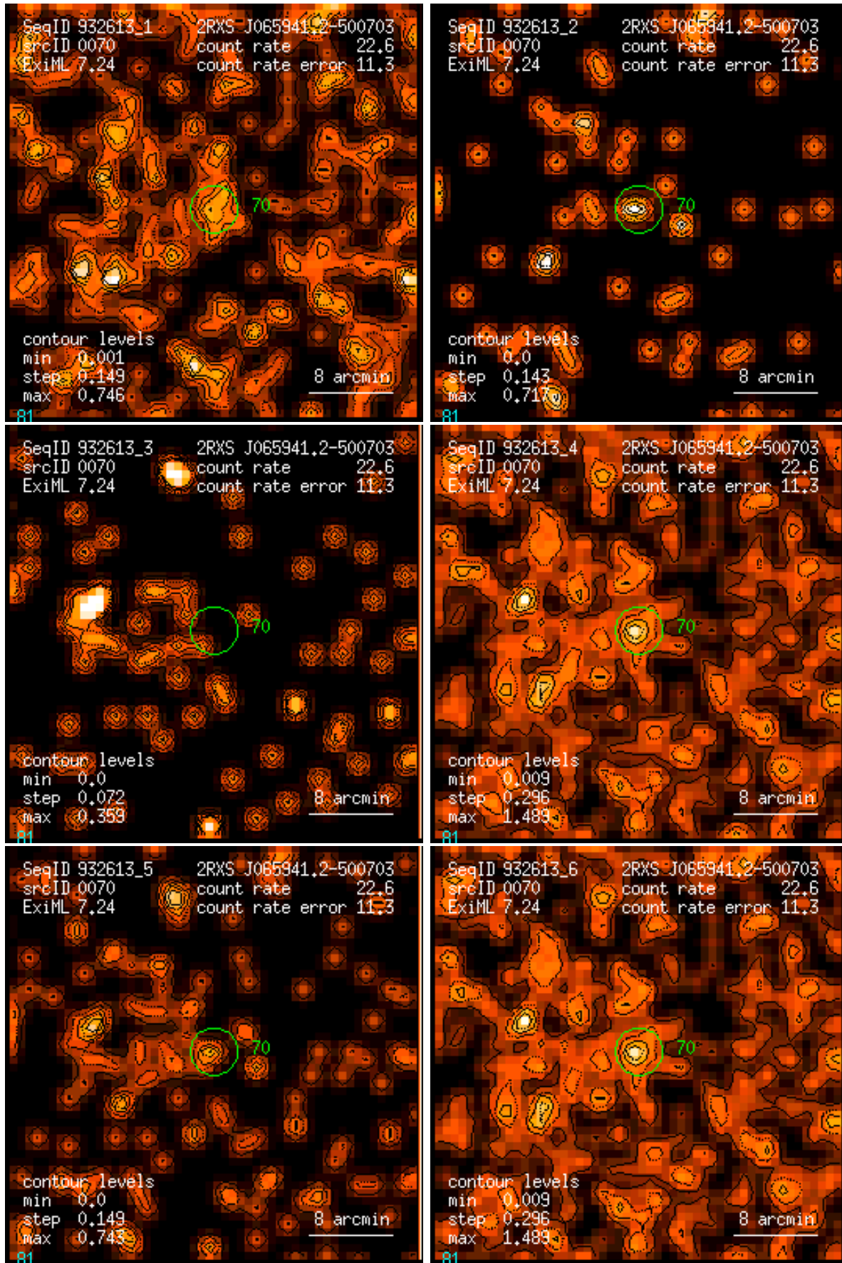
Figure 70: RASS 932613: detection 0070: band rate images, Gaussian filter: (1) PSPC channels 11 – 41, (2) 52 – 90, (3) 91 – 201, (4) 11 – 235, (5) 52 – 201, (6) 11 – 201. Broad band rates in counts/ks. Band rate contour levels in counts/ks/arcmin 2 .
