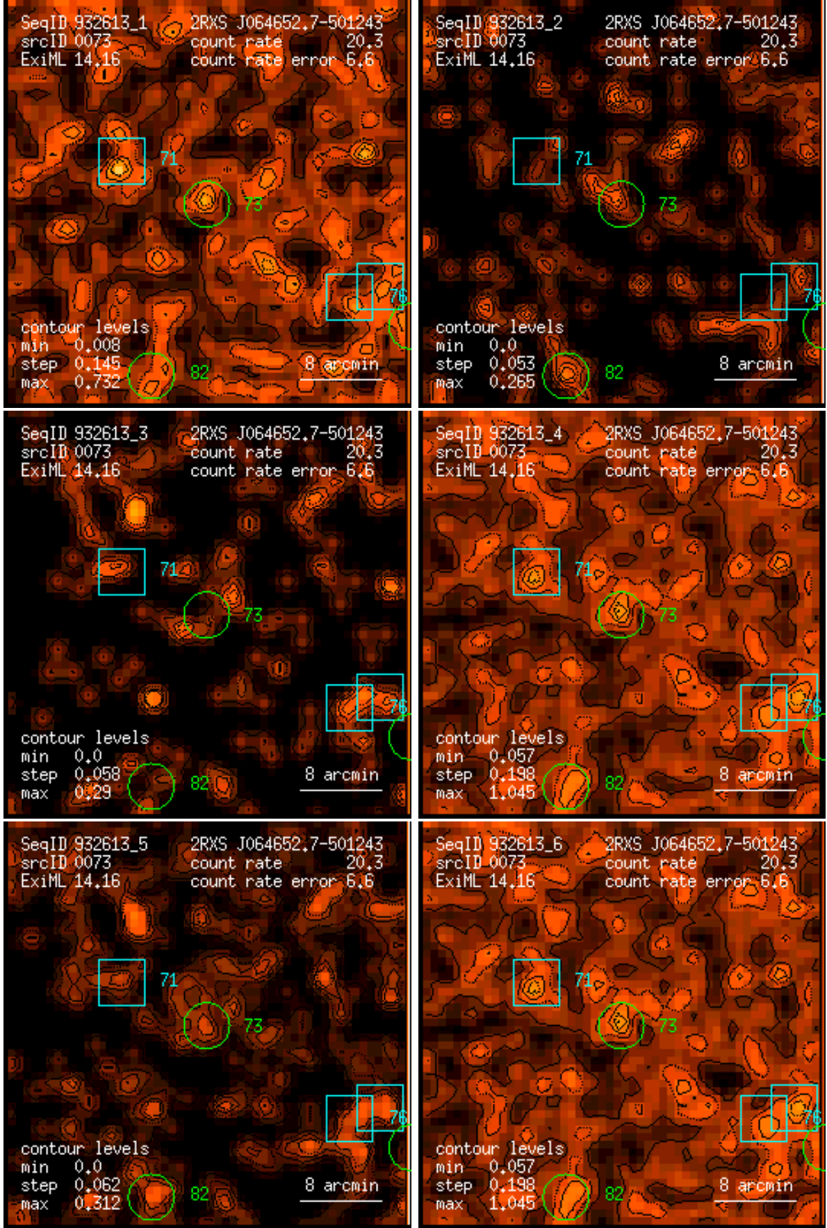
Figure 73: RASS 932613: detection 0073: band rate images, Gaussian filter: (1) PSPC channels 11 – 41, (2) 52 – 90, (3) 91 – 201, (4) 11 – 235, (5) 52 – 201, (6) 11 – 201. Broad band rates in counts/ks. Band rate contour levels in counts/ks/arcmin 2 .
