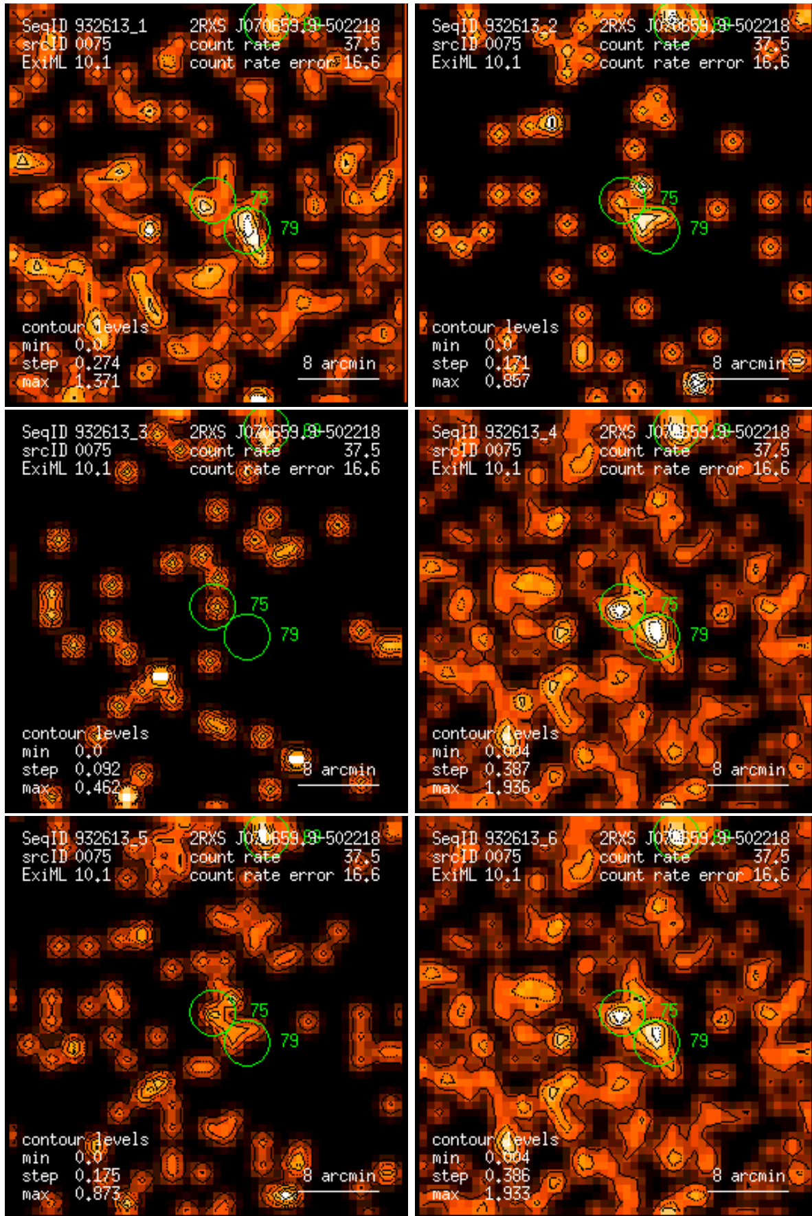
Figure 75: RASS 932613: detection 0075: band rate images, Gaussian filter: (1) PSPC channels 11 – 41, (2) 52 – 90, (3) 91 – 201, (4) 11 – 235, (5) 52 – 201, (6) 11 – 201. Broad band rates in counts/ks. Band rate contour levels in counts/ks/arcmin 2 .
