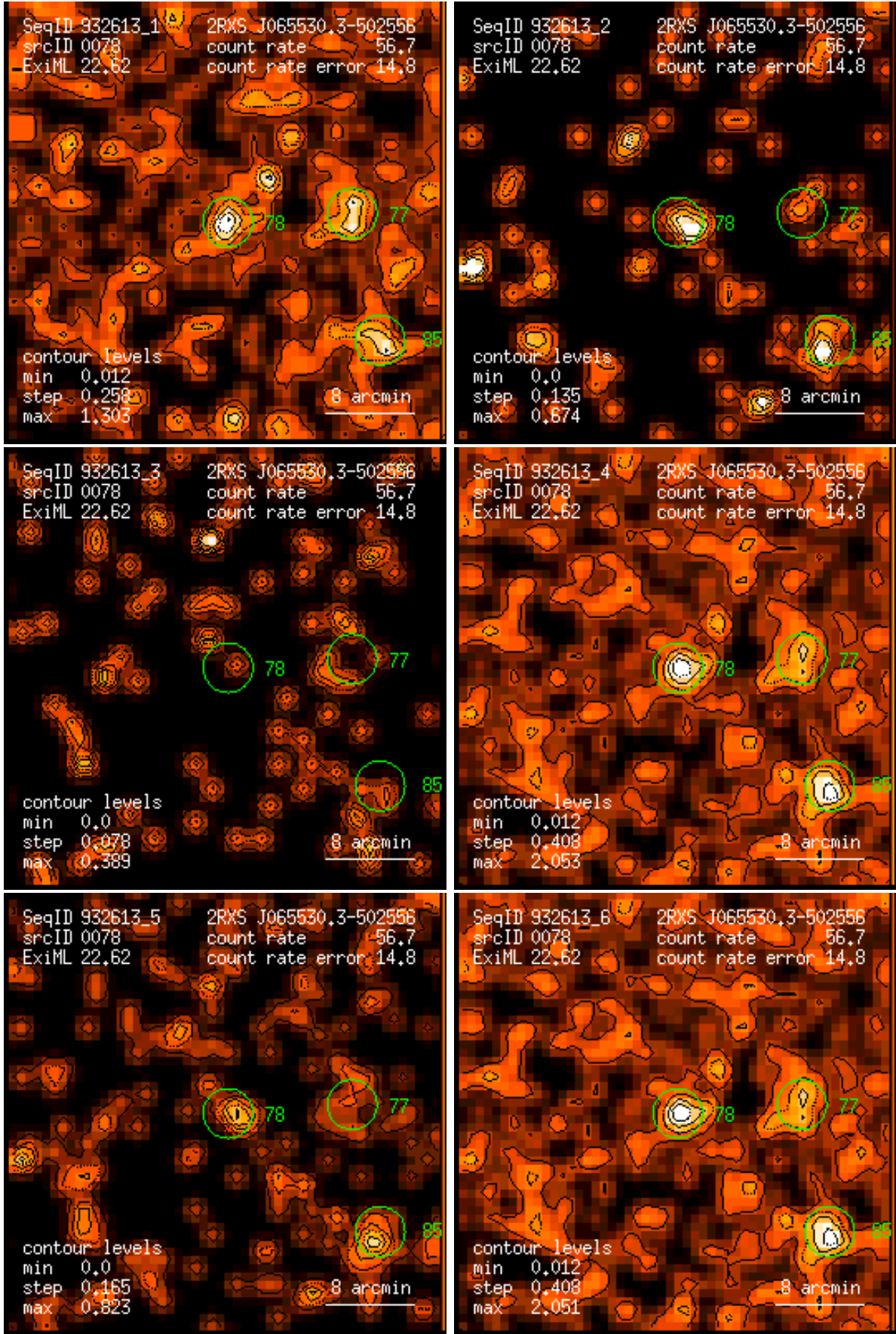
Figure 78: RASS 932613: detection 0078: band rate images, Gaussian filter: (1) PSPC channels 11 – 41, (2) 52 – 90, (3) 91 – 201, (4) 11 – 235, (5) 52 – 201, (6) 11 – 201. Broad band rates in counts/ks. Band rate contour levels in counts/ks/arcmin 2 .
