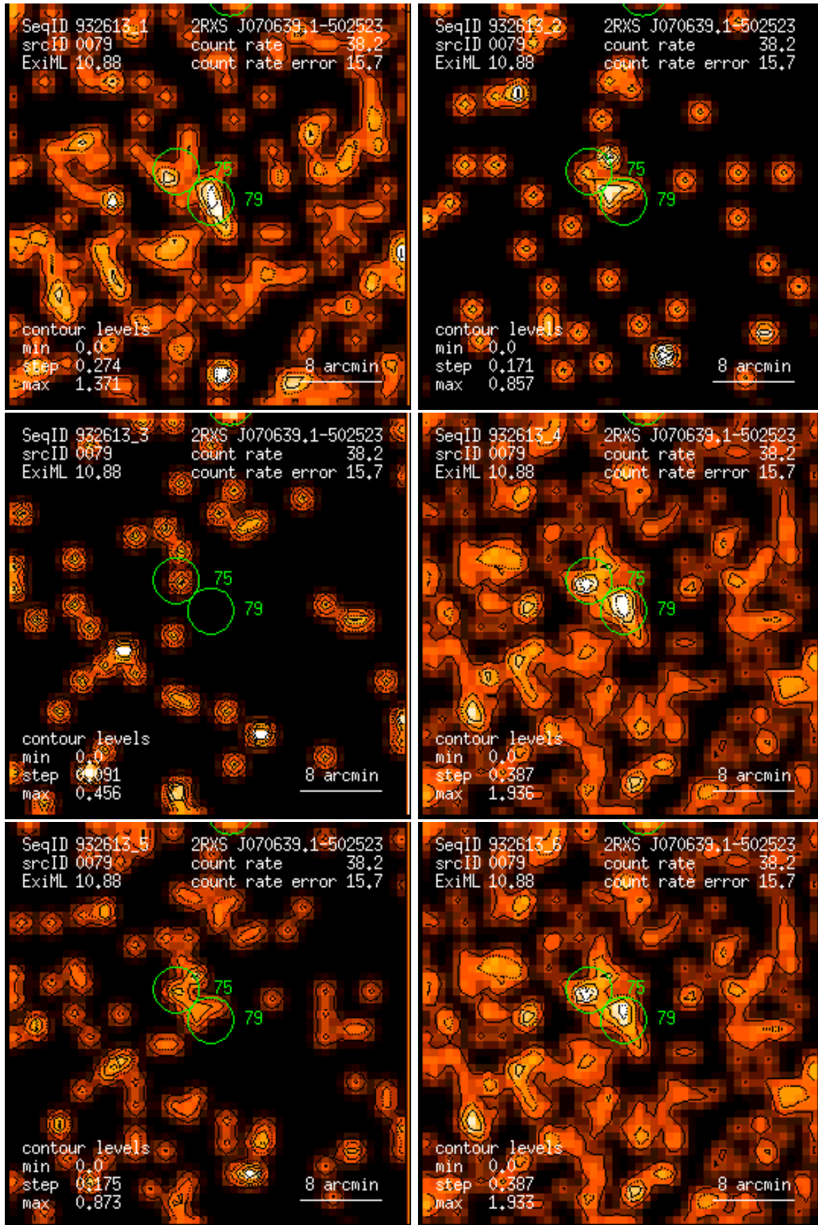
Figure 79: RASS 932613: detection 0079: band rate images, Gaussian filter: (1) PSPC channels 11 – 41, (2) 52 – 90, (3) 91 – 201, (4) 11 – 235, (5) 52 – 201, (6) 11 – 201. Broad band rates in counts/ks. Band rate contour levels in counts/ks/arcmin 2 .
