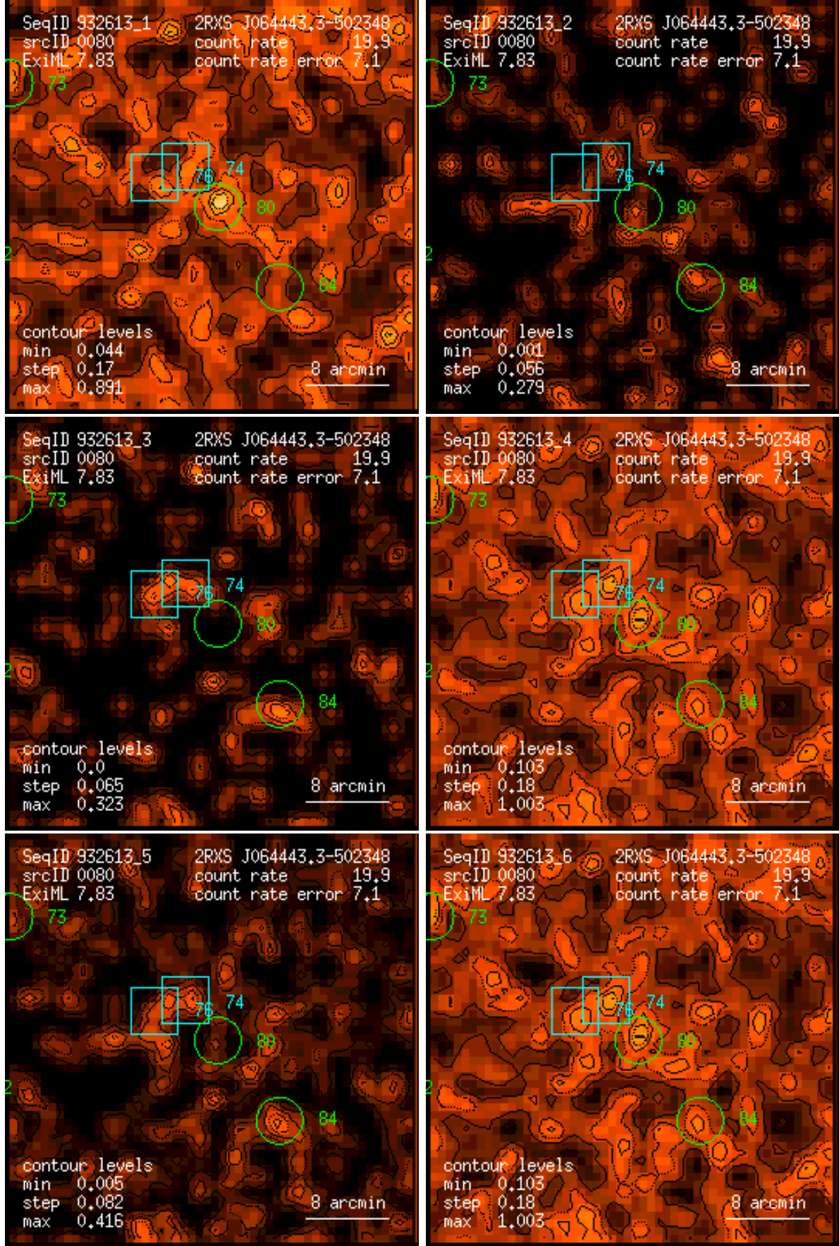
Figure 80: RASS 932613: detection 0080: band rate images, Gaussian filter: (1) PSPC channels 11 – 41, (2) 52 – 90, (3) 91 – 201, (4) 11 – 235, (5) 52 – 201, (6) 11 – 201. Broad band rates in counts/ks. Band rate contour levels in counts/ks/arcmin 2 .
