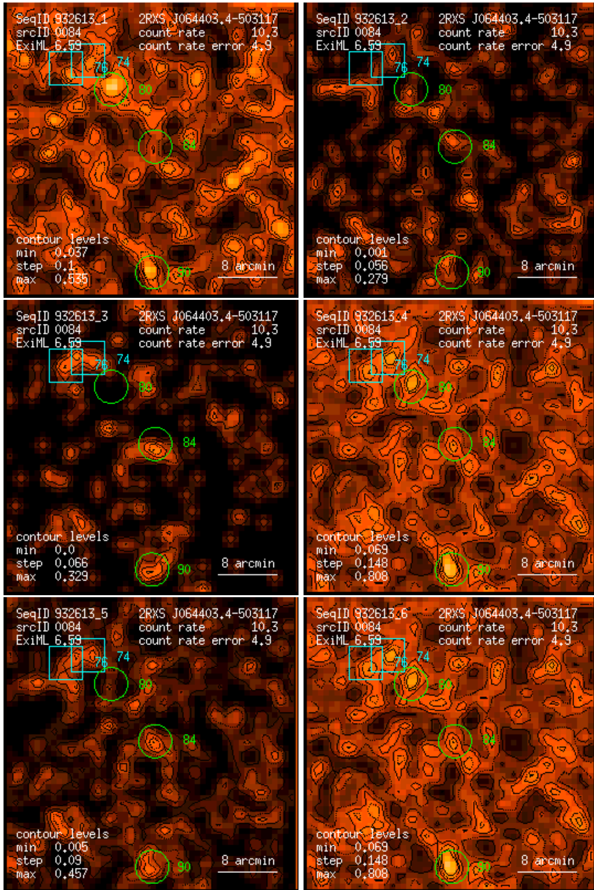
Figure 84: RASS 932613: detection 0084: band rate images, Gaussian filter: (1) PSPC channels 11 – 41, (2) 52 – 90, (3) 91 – 201, (4) 11 – 235, (5) 52 – 201, (6) 11 – 201. Broad band rates in counts/ks. Band rate contour levels in counts/ks/arcmin 2 .
