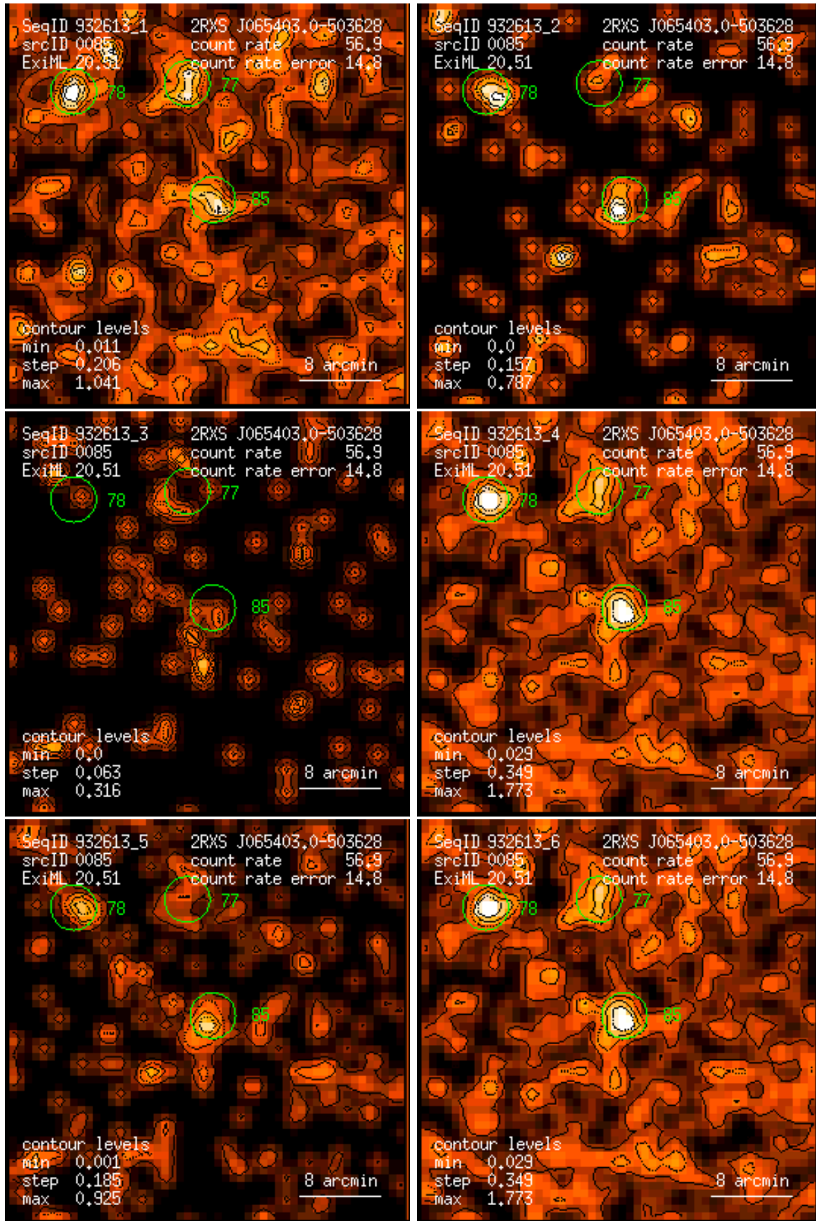
Figure 85: RASS 932613: detection 0085: band rate images, Gaussian filter: (1) PSPC channels 11 – 41, (2) 52 – 90, (3) 91 – 201, (4) 11 – 235, (5) 52 – 201, (6) 11 – 201. Broad band rates in counts/ks. Band rate contour levels in counts/ks/arcmin 2 .
