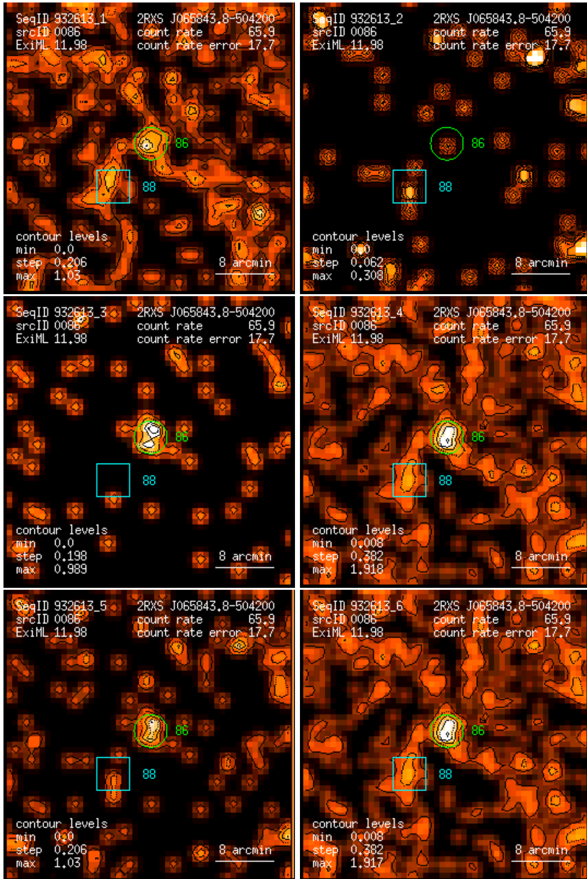
Figure 86: RASS 932613: detection 0086: band rate images, Gaussian filter: (1) PSPC channels 11 – 41, (2) 52 – 90, (3) 91 – 201, (4) 11 – 235, (5) 52 – 201, (6) 11 – 201. Broad band rates in counts/ks. Band rate contour levels in counts/ks/arcmin 2 .
