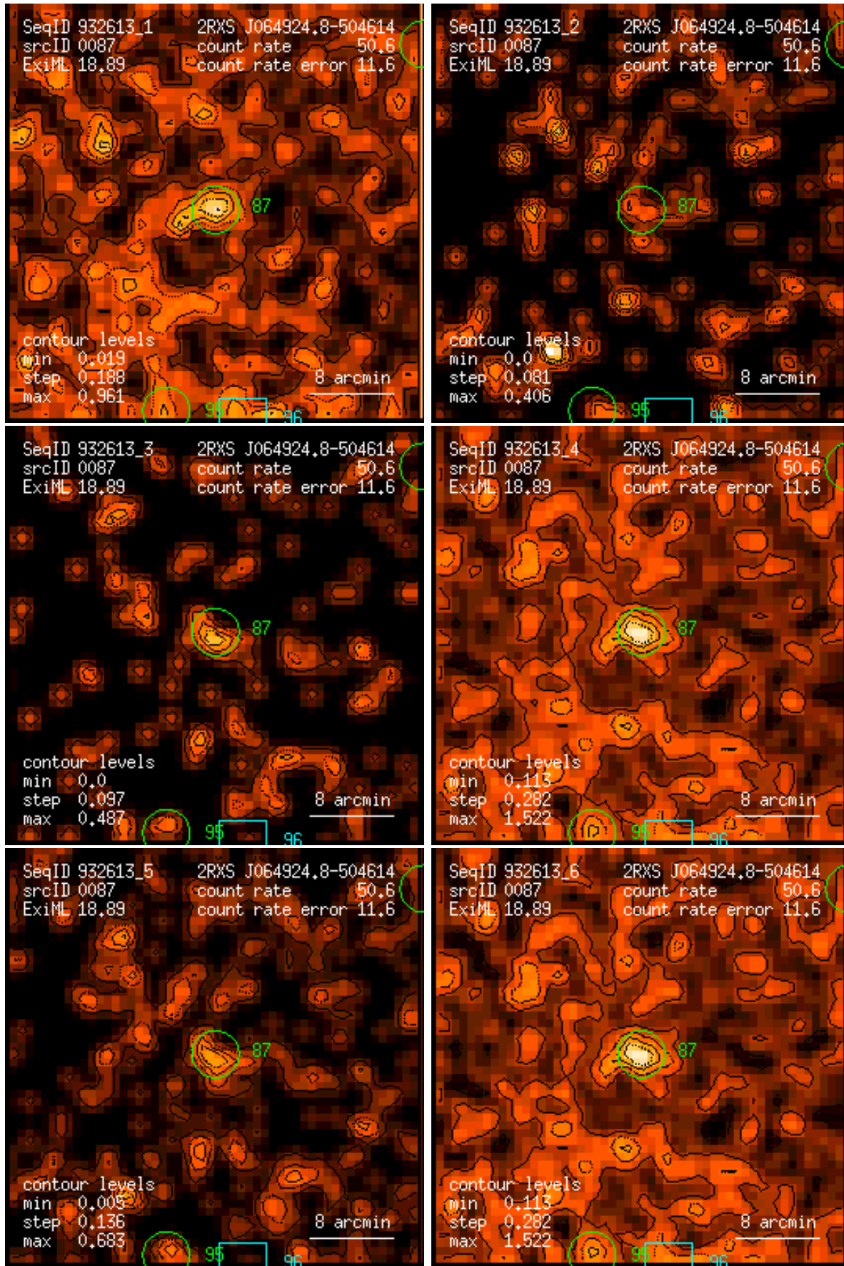
Figure 87: RASS 932613: detection 0087: band rate images, Gaussian filter: (1) PSPC channels 11 – 41, (2) 52 – 90, (3) 91 – 201, (4) 11 – 235, (5) 52 – 201, (6) 11 – 201. Broad band rates in counts/ks. Band rate contour levels in counts/ks/arcmin 2 .
