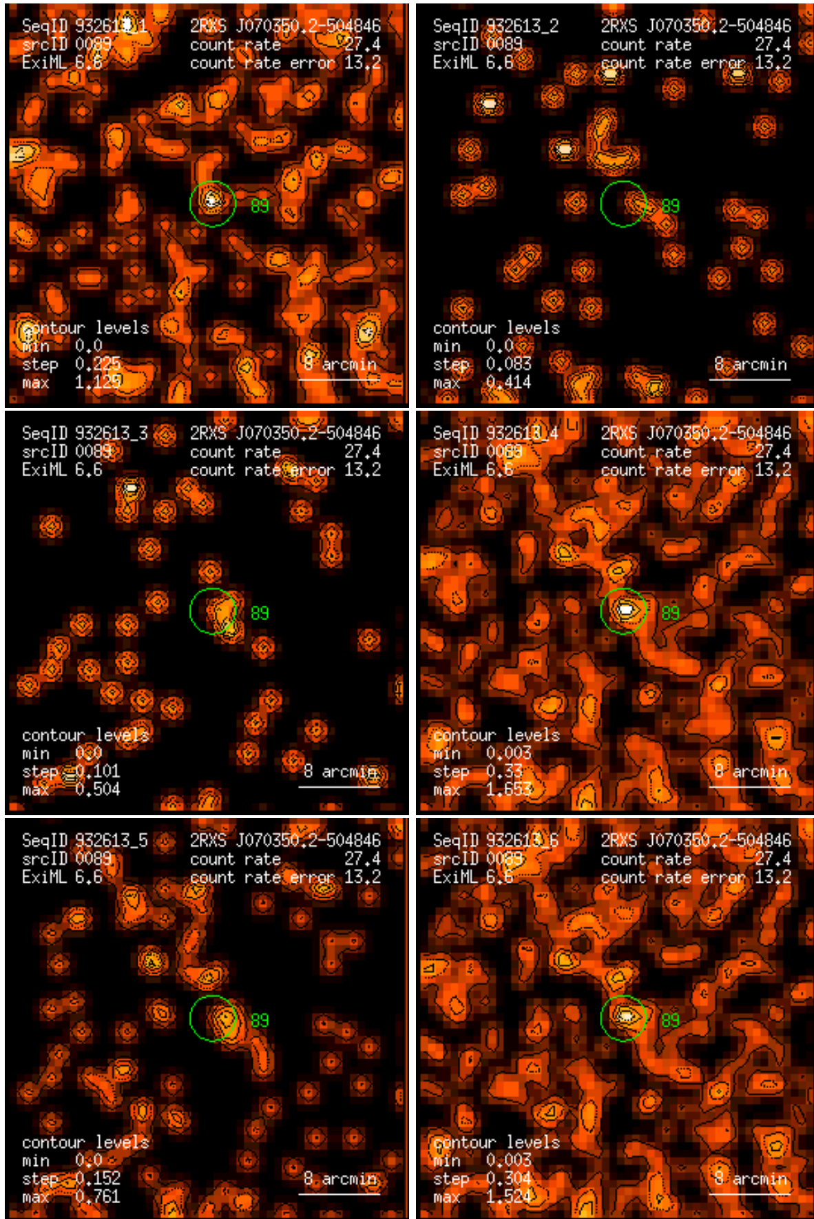
Figure 89: RASS 932613: detection 0089: band rate images, Gaussian filter: (1) PSPC channels 11 – 41, (2) 52 – 90, (3) 91 – 201, (4) 11 – 235, (5) 52 – 201, (6) 11 – 201. Broad band rates in counts/ks. Band rate contour levels in counts/ks/arcmin 2 .
