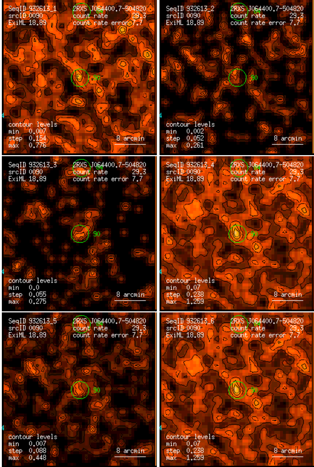
Figure 90: RASS 932613: detection 0090: band rate images, Gaussian filter: (1) PSPC channels 11 – 41, (2) 52 – 90, (3) 91 – 201, (4) 11 – 235, (5) 52 – 201, (6) 11 – 201. Broad band rates in counts/ks. Band rate contour levels in counts/ks/arcmin 2 .
