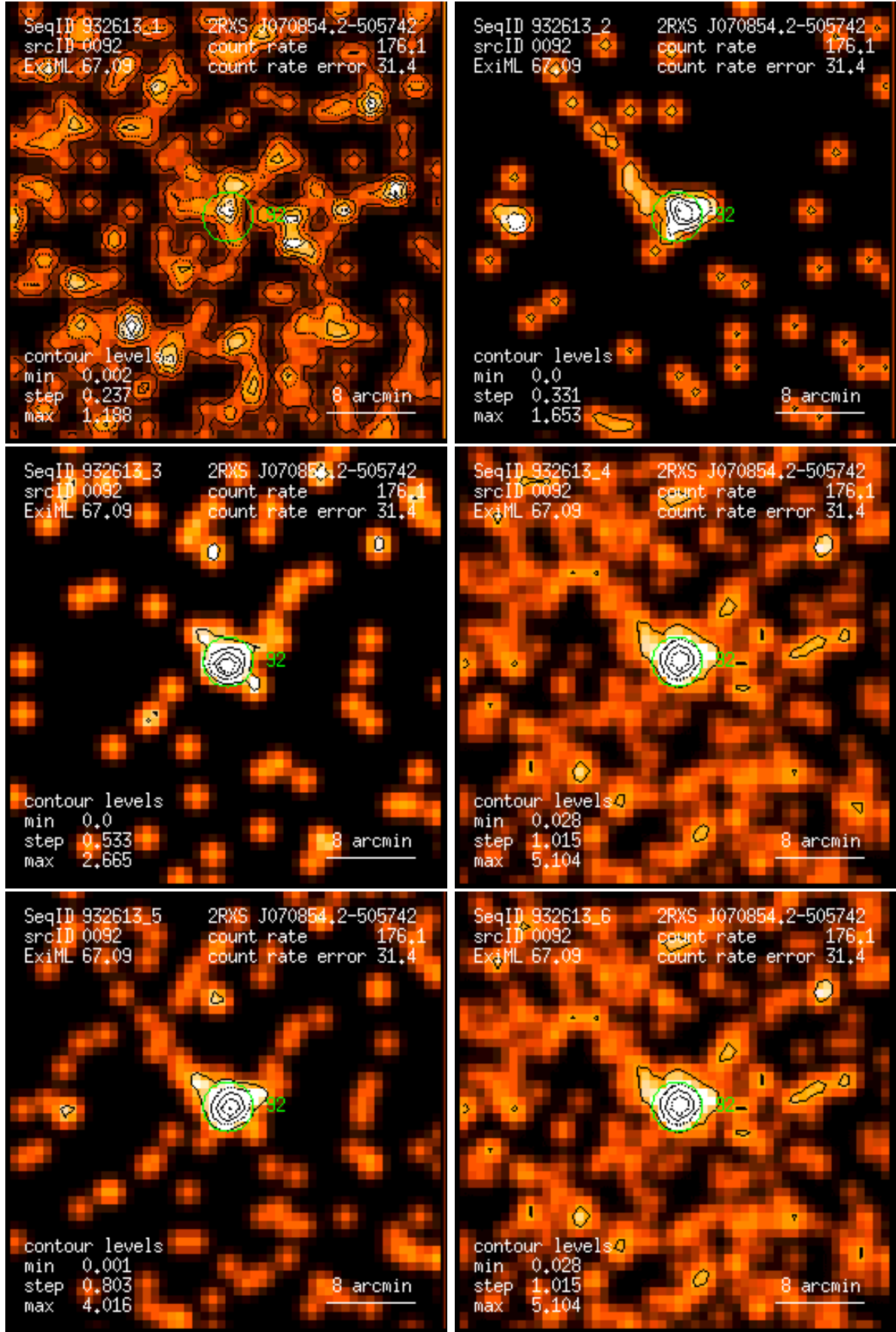
Figure 92: RASS 932613: detection 0092: band rate images, Gaussian filter: (1) PSPC channels 11 – 41, (2) 52 – 90, (3) 91 – 201, (4) 11 – 235, (5) 52 – 201, (6) 11 – 201. Broad band rates in counts/ks. Band rate contour levels in counts/ks/arcmin 2 .
