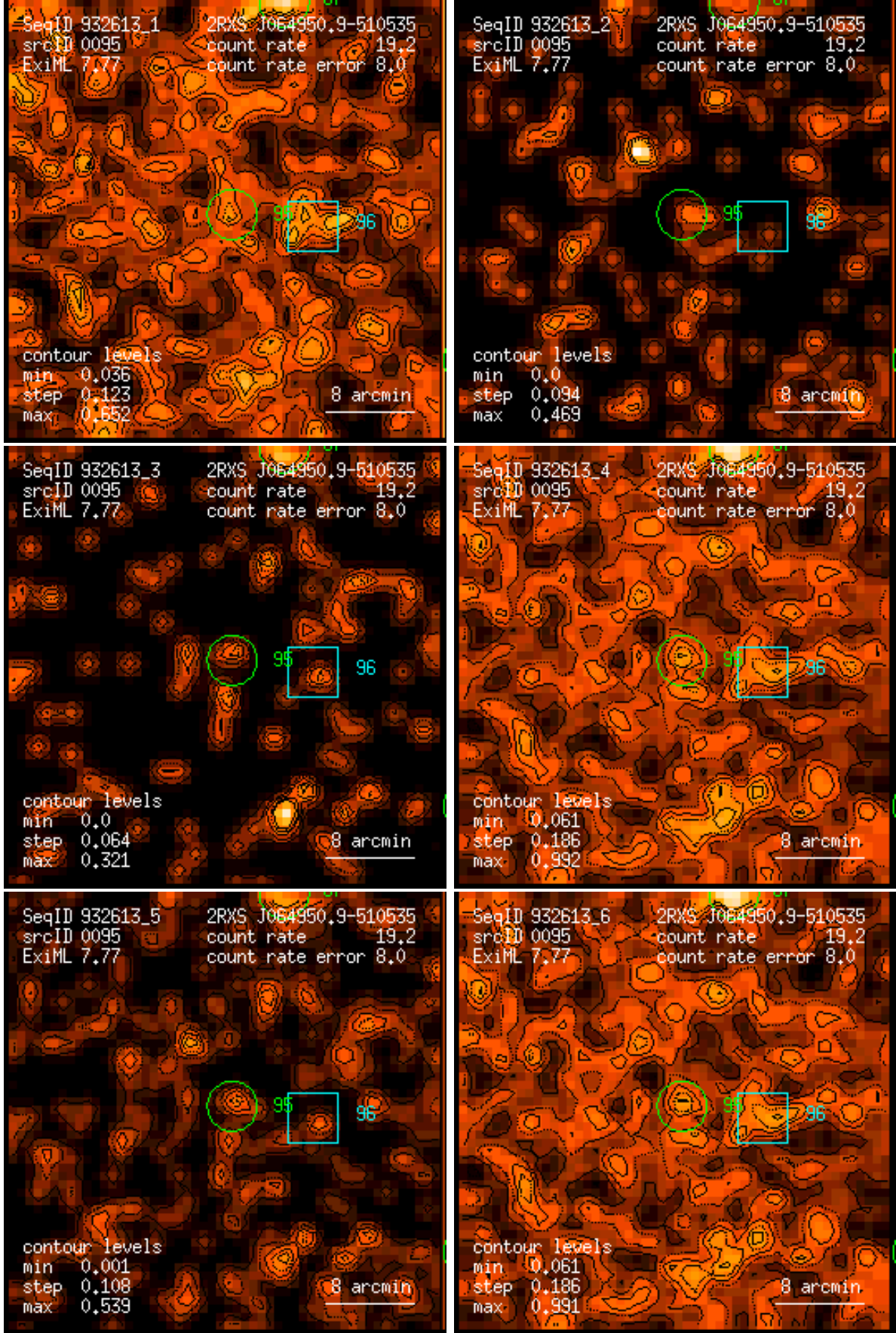
Figure 95: RASS 932613: detection 0095: band rate images, Gaussian filter: (1) PSPC channels 11 – 41, (2) 52 – 90, (3) 91 – 201, (4) 11 – 235, (5) 52 – 201, (6) 11 – 201. Broad band rates in counts/ks. Band rate contour levels in counts/ks/arcmin 2 .
