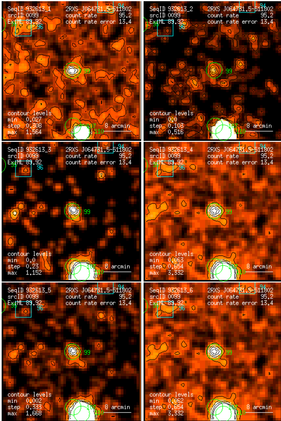
Figure 99: RASS 932613: detection 0099: band rate images, Gaussian filter: (1) PSPC channels 11 – 41, (2) 52 – 90, (3) 91 – 201, (4) 11 – 235, (5) 52 – 201, (6) 11 – 201. Broad band rates in counts/ks. Band rate contour levels in counts/ks/arcmin 2 .
