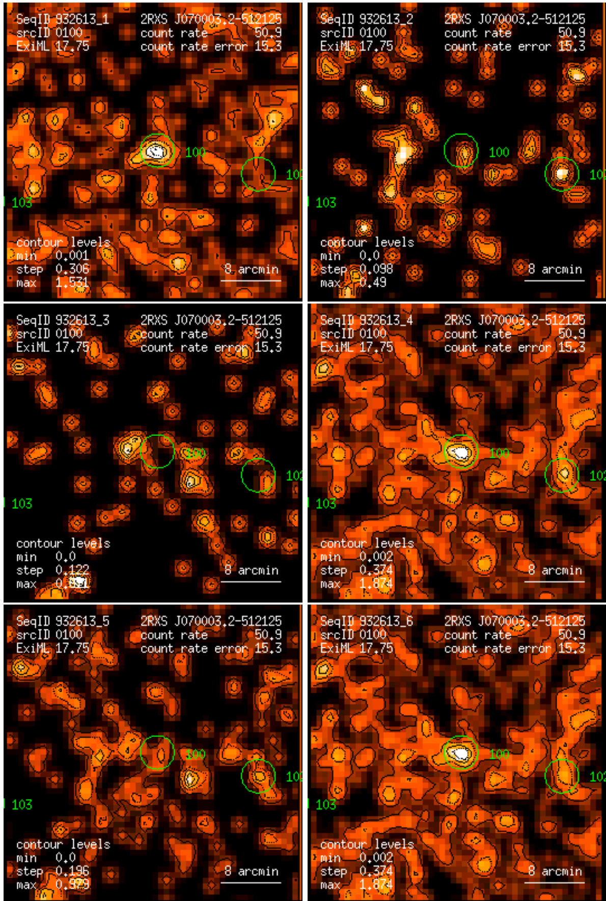
Figure 100: RASS 932613: detection 0100: band rate images, Gaussian filter: (1) PSPC channels 11 – 41, (2) 52 – 90, (3) 91 – 201, (4) 11 – 235, (5) 52 – 201, (6) 11 – 201. Broad band rates in counts/ks. Band rate contour levels in counts/ks/arcmin 2 .
