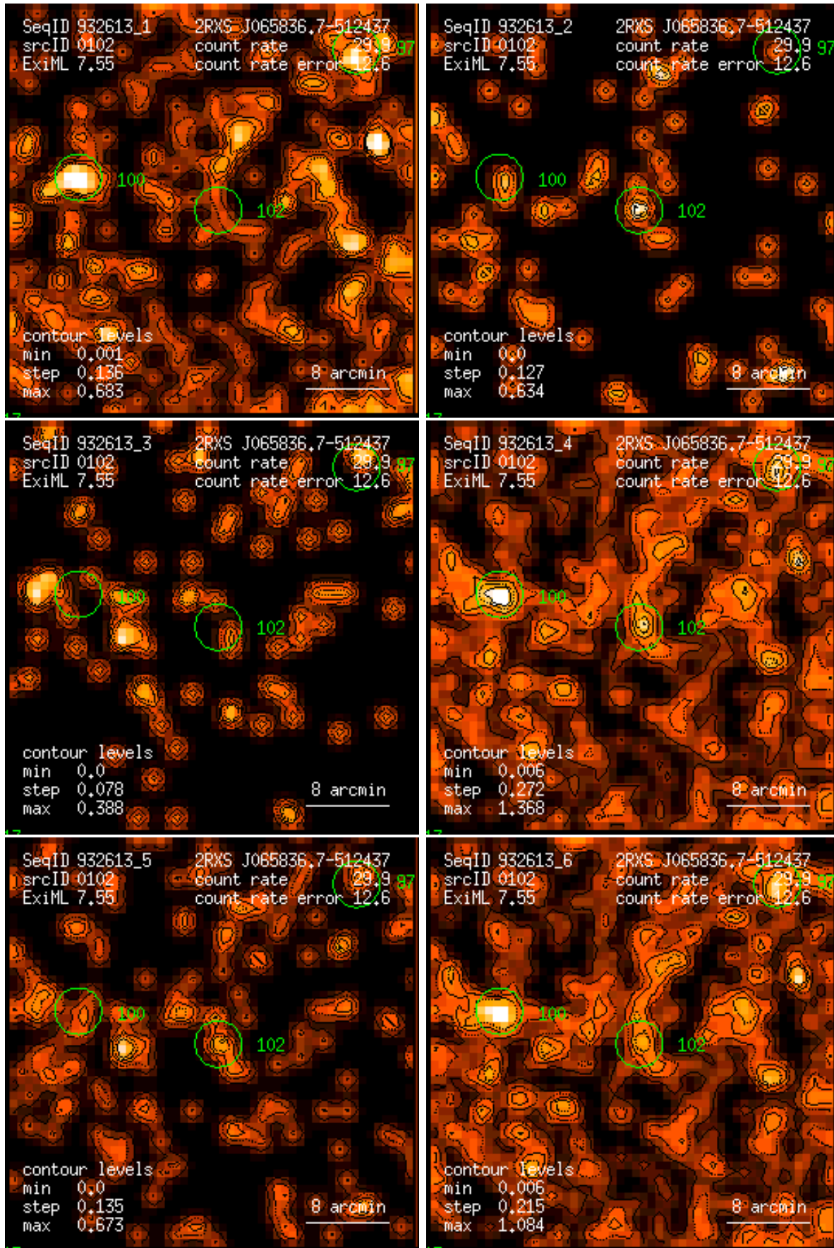
Figure 102: RASS 932613: detection 0102: band rate images, Gaussian filter: (1) PSPC channels 11 – 41, (2) 52 – 90, (3) 91 – 201, (4) 11 – 235, (5) 52 – 201, (6) 11 – 201. Broad band rates in counts/ks. Band rate contour levels in counts/ks/arcmin 2 .
