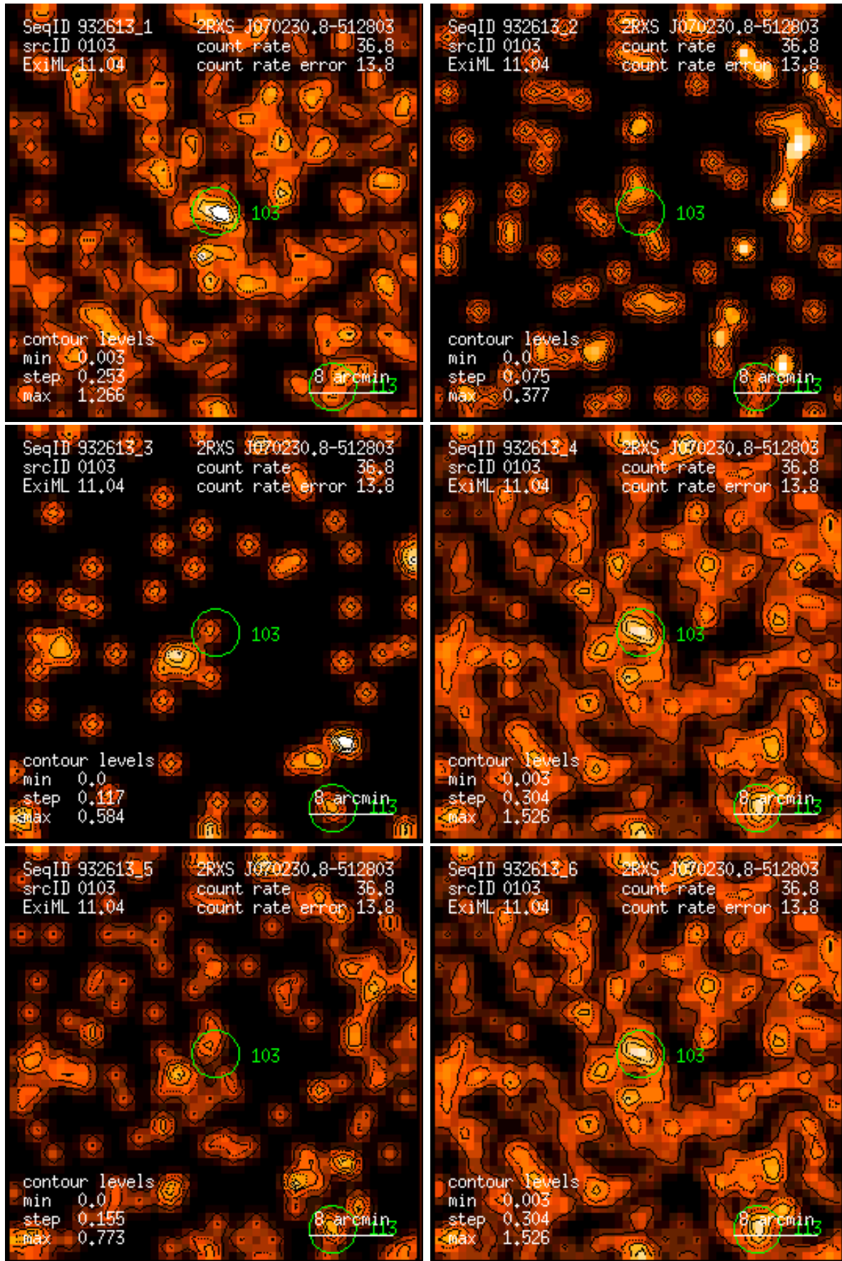
Figure 103: RASS 932613: detection 0103: band rate images, Gaussian filter: (1) PSPC channels 11 – 41, (2) 52 – 90, (3) 91 – 201, (4) 11 – 235, (5) 52 – 201, (6) 11 – 201. Broad band rates in counts/ks. Band rate contour levels in counts/ks/arcmin 2 .
