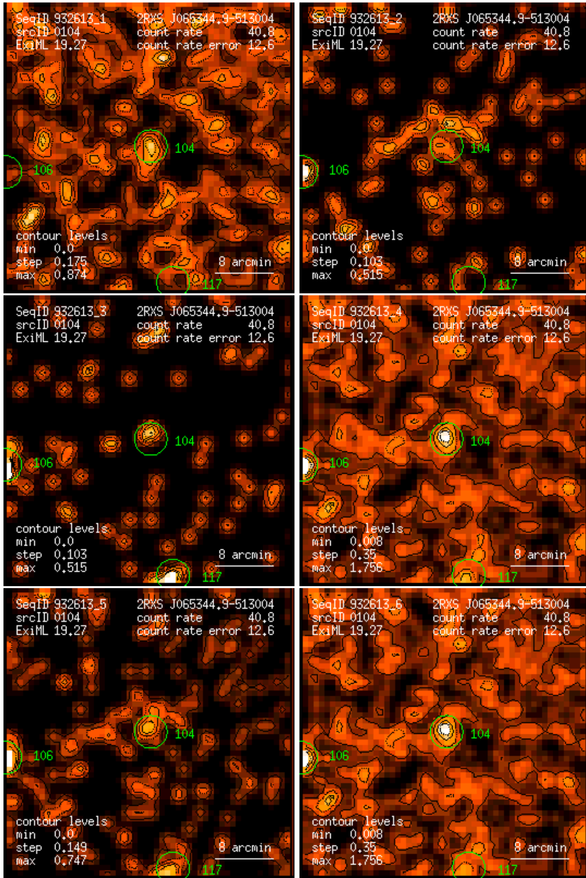
Figure 104: RASS 932613: detection 0104: band rate images, Gaussian filter: (1) PSPC channels 11 – 41, (2) 52 – 90, (3) 91 – 201, (4) 11 – 235, (5) 52 – 201, (6) 11 – 201. Broad band rates in counts/ks. Band rate contour levels in counts/ks/arcmin 2 .
