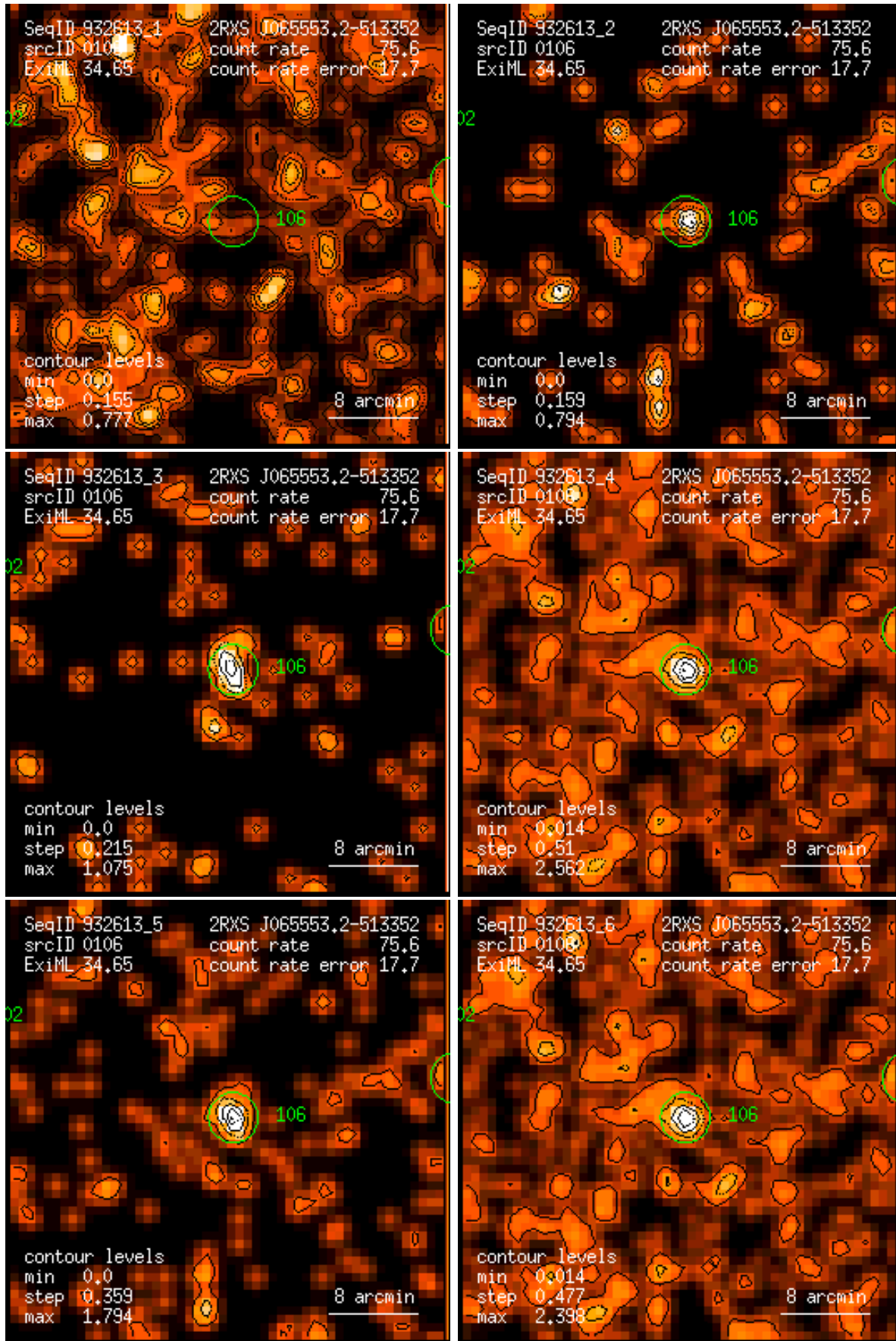
Figure 106: RASS 932613: detection 0106: band rate images, Gaussian filter: (1) PSPC channels 11 – 41, (2) 52 – 90, (3) 91 – 201, (4) 11 – 235, (5) 52 – 201, (6) 11 – 201. Broad band rates in counts/ks. Band rate contour levels in counts/ks/arcmin 2 .
