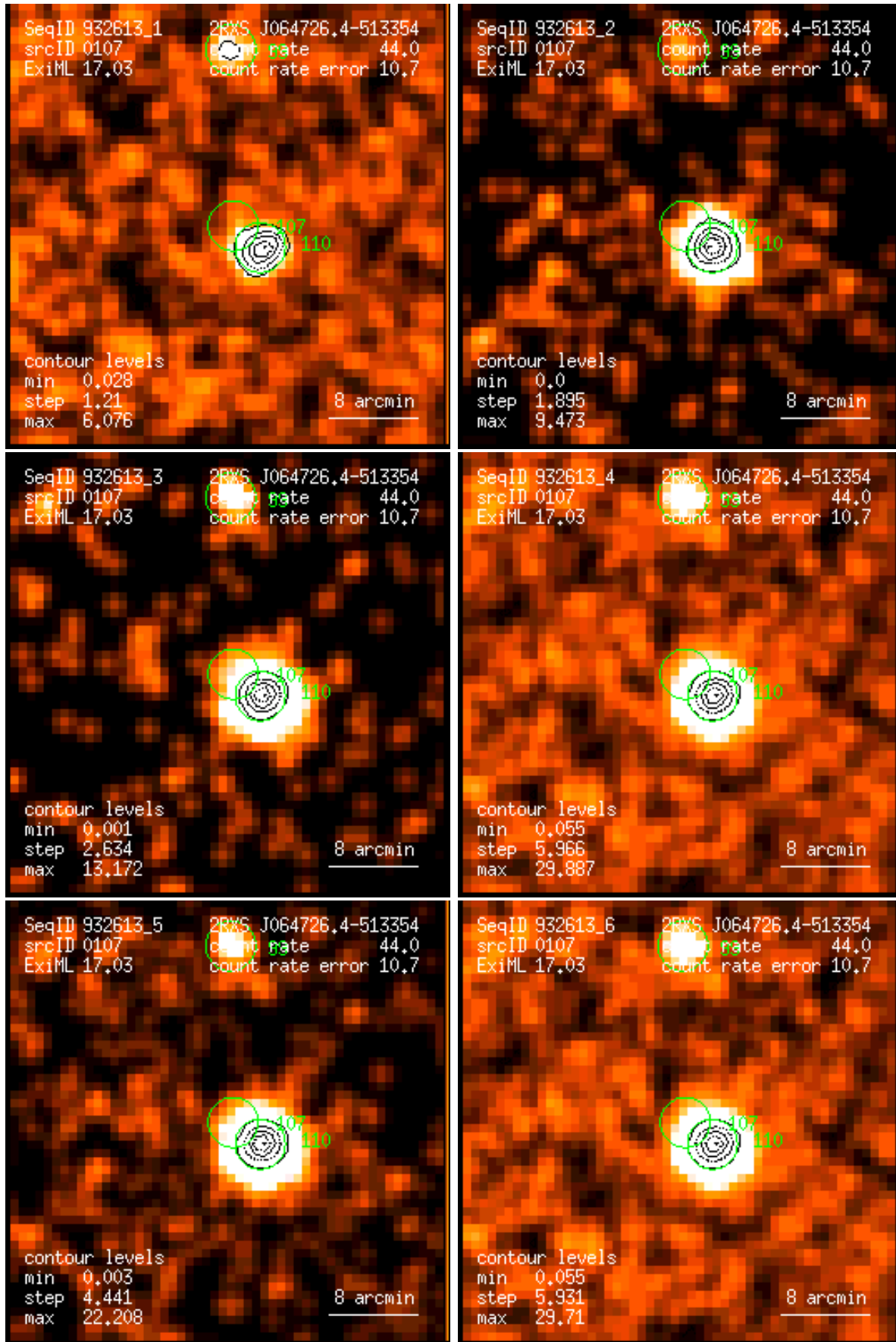
Figure 107: RASS 932613: detection 0107: band rate images, Gaussian filter: (1) PSPC channels 11 – 41, (2) 52 – 90, (3) 91 – 201, (4) 11 – 235, (5) 52 – 201, (6) 11 – 201. Broad band rates in counts/ks. Band rate contour levels in counts/ks/arcmin 2 .
