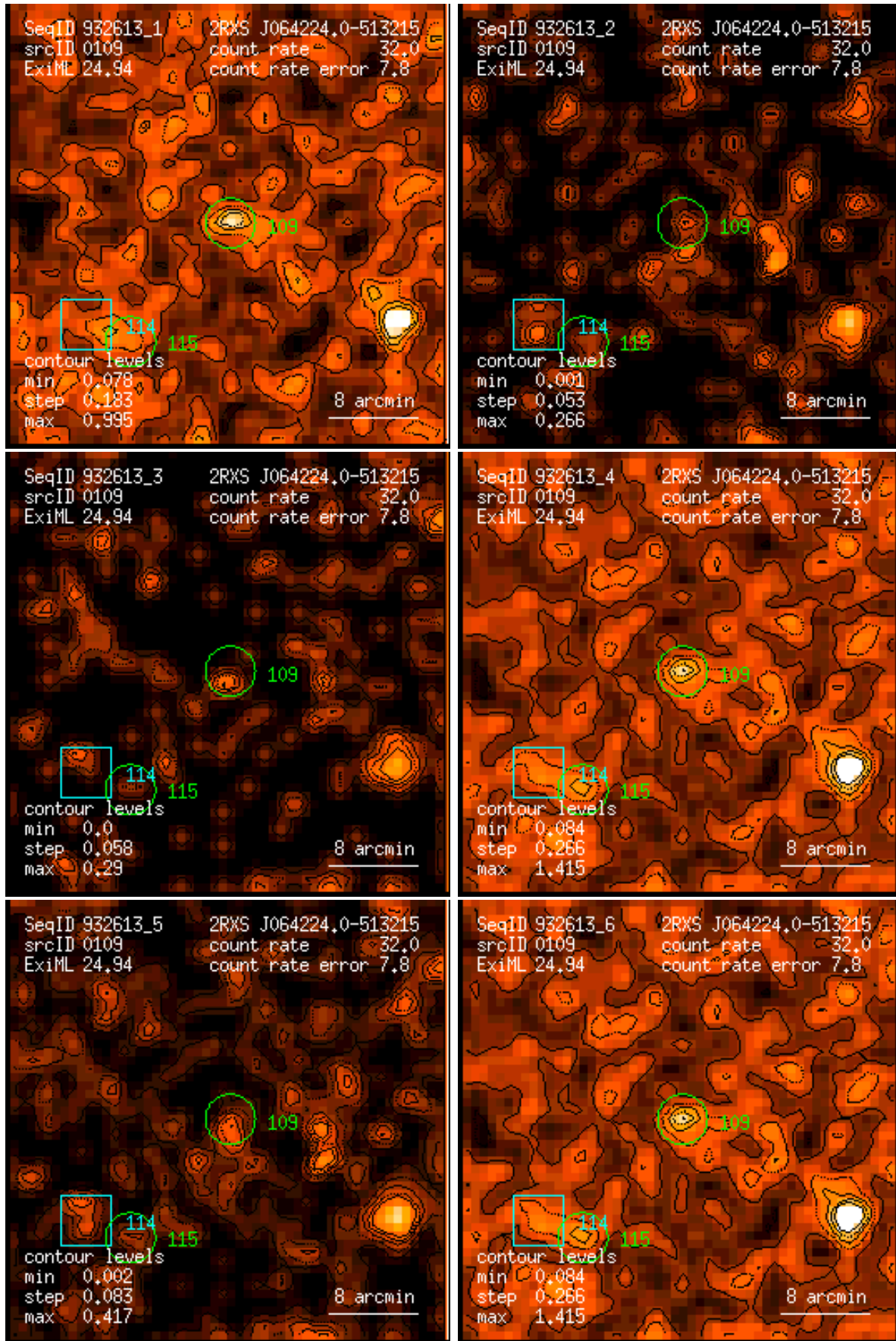
Figure 109: RASS 932613: detection 0109: band rate images, Gaussian filter: (1) PSPC channels 11 – 41, (2) 52 – 90, (3) 91 – 201, (4) 11 – 235, (5) 52 – 201, (6) 11 – 201. Broad band rates in counts/ks. Band rate contour levels in counts/ks/arcmin 2 .
