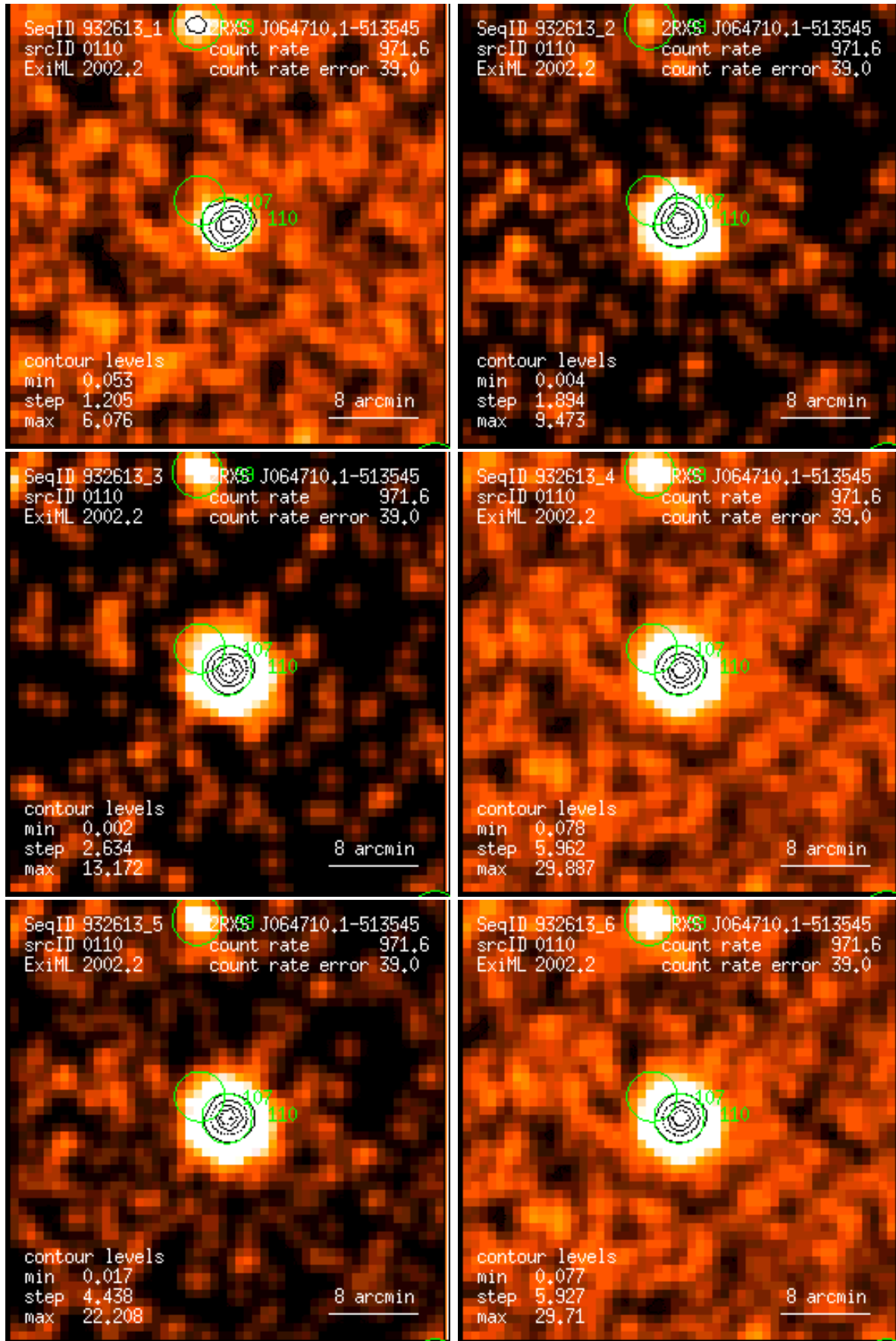
Figure 110: RASS 932613: detection 0110: band rate images, Gaussian filter: (1) PSPC channels 11 – 41, (2) 52 – 90, (3) 91 – 201, (4) 11 – 235, (5) 52 – 201, (6) 11 – 201. Broad band rates in counts/ks. Band rate contour levels in counts/ks/arcmin 2 .
