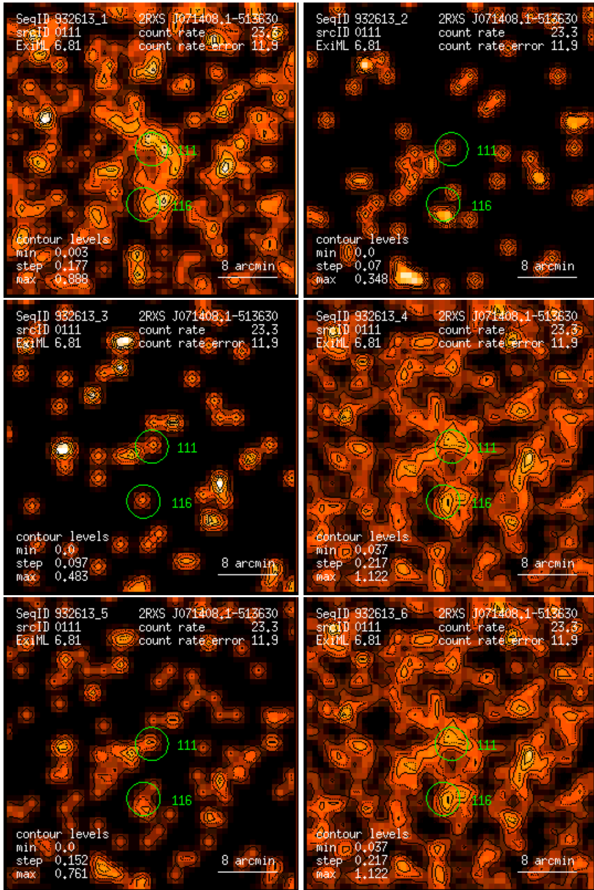
Figure 111: RASS 932613: detection 0111: band rate images, Gaussian filter: (1) PSPC channels 11 – 41, (2) 52 – 90, (3) 91 – 201, (4) 11 – 235, (5) 52 – 201, (6) 11 – 201. Broad band rates in counts/ks. Band rate contour levels in counts/ks/arcmin 2 .
