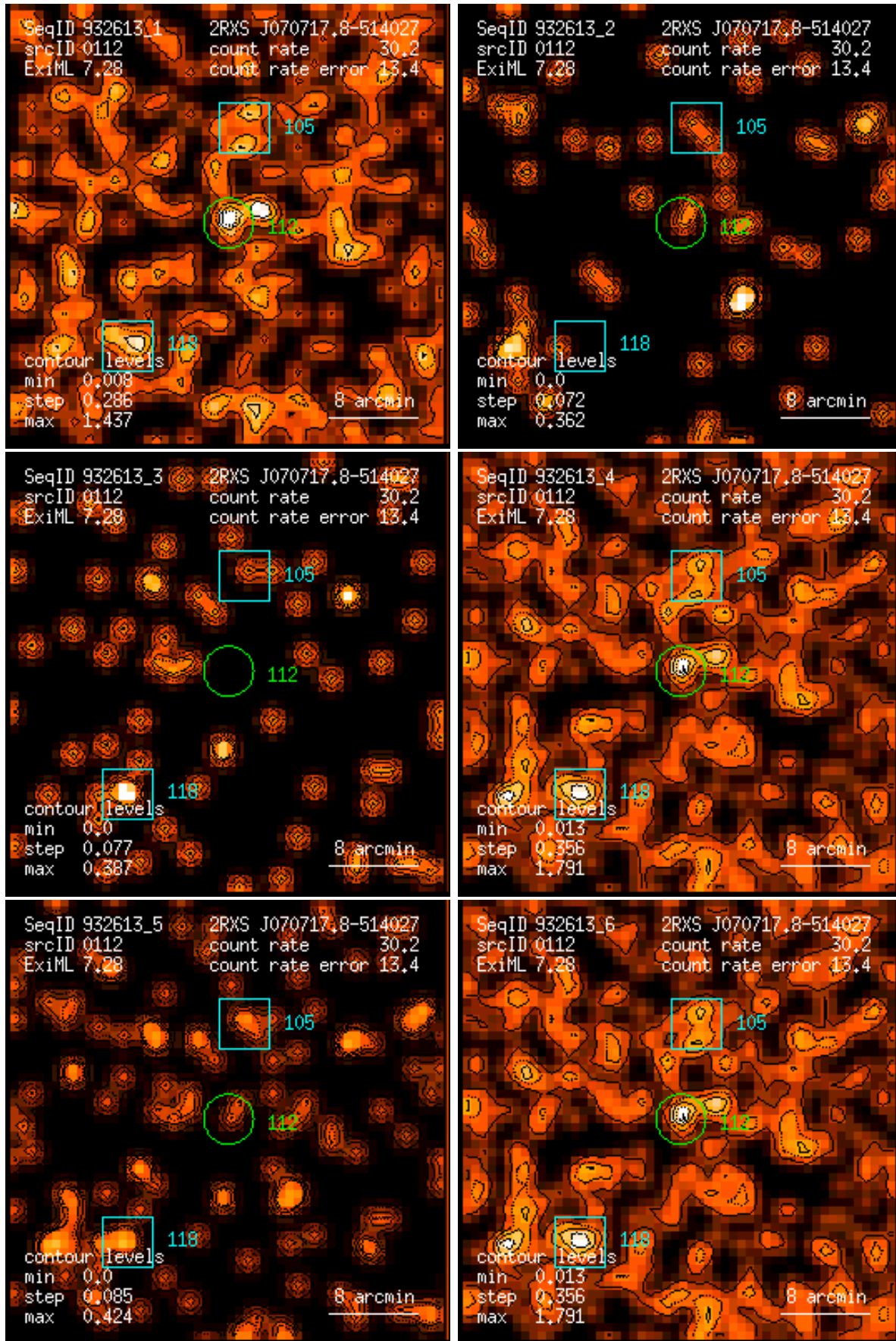
Figure 112: RASS 932613: detection 0112: band rate images, Gaussian filter: (1) PSPC channels 11 – 41, (2) 52 – 90, (3) 91 – 201, (4) 11 – 235, (5) 52 – 201, (6) 11 – 201. Broad band rates in counts/ks. Band rate contour levels in counts/ks/arcmin 2 .
