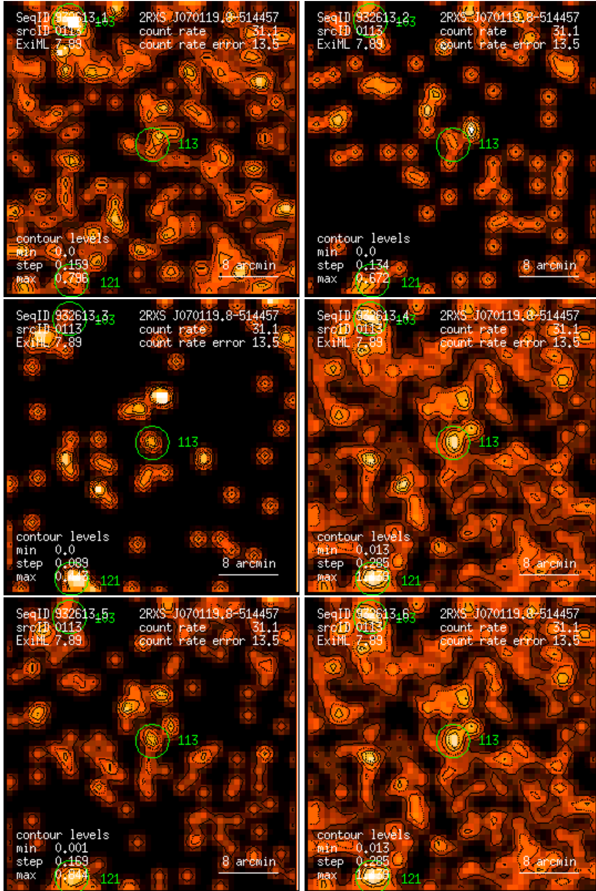
Figure 113: RASS 932613: detection 0113: band rate images, Gaussian filter: (1) PSPC channels 11 – 41, (2) 52 – 90, (3) 91 – 201, (4) 11 – 235, (5) 52 – 201, (6) 11 – 201. Broad band rates in counts/ks. Band rate contour levels in counts/ks/arcmin 2 .
