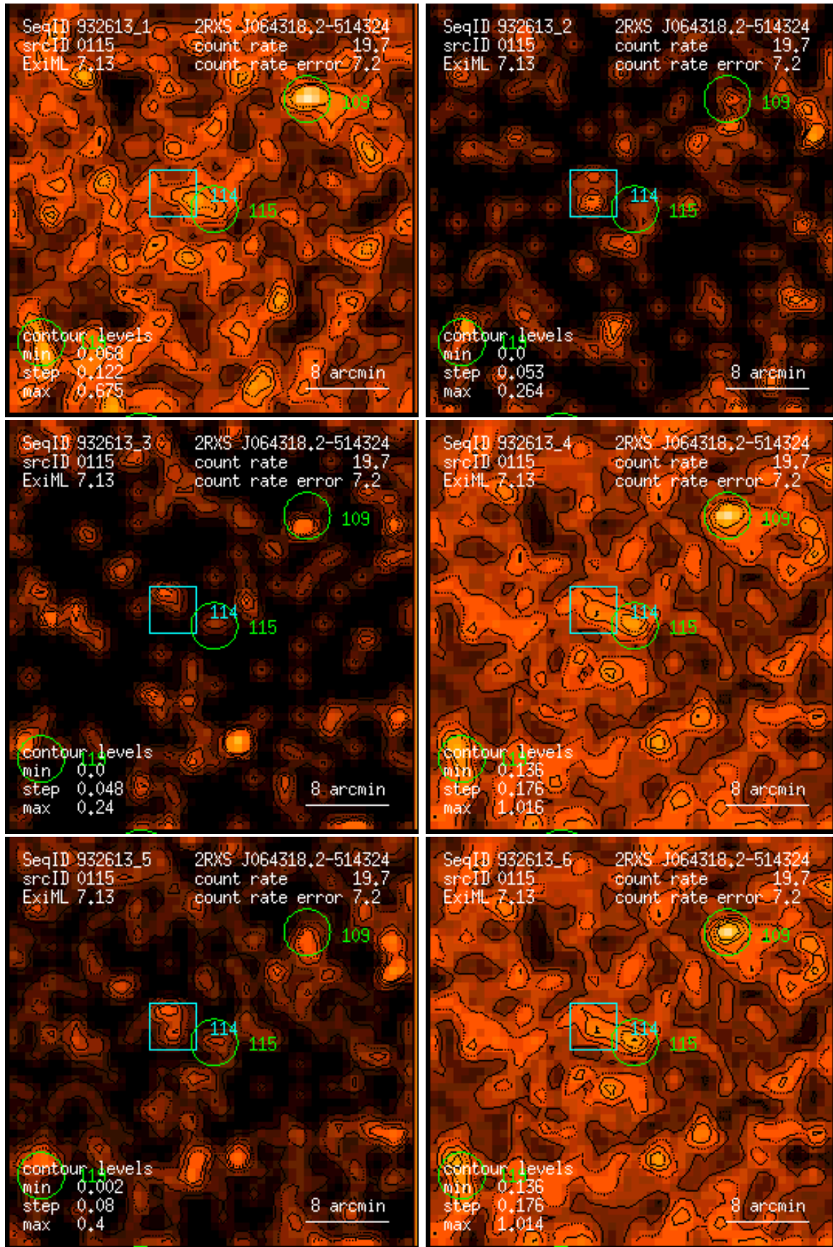
Figure 115: RASS 932613: detection 0115: band rate images, Gaussian filter: (1) PSPC channels 11 – 41, (2) 52 – 90, (3) 91 – 201, (4) 11 – 235, (5) 52 – 201, (6) 11 – 201. Broad band rates in counts/ks. Band rate contour levels in counts/ks/arcmin 2 .
