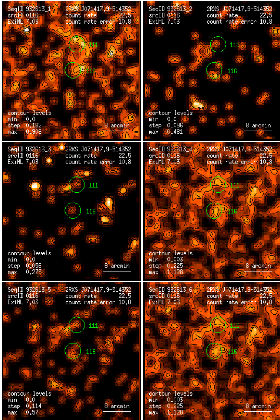
Figure 116: RASS 932613: detection 0116: band rate images, Gaussian filter: (1) PSPC channels 11 – 41, (2) 52 – 90, (3) 91 – 201, (4) 11 – 235, (5) 52 – 201, (6) 11 – 201. Broad band rates in counts/ks. Band rate contour levels in counts/ks/arcmin 2 .
